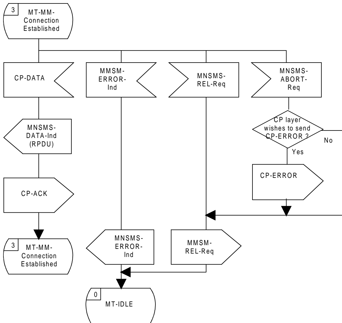
MT-SMC-entity on Network-side Message transfer active SDL-12
