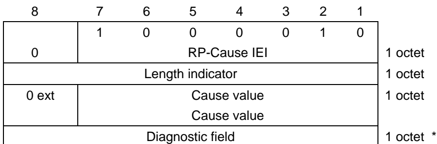
Figure 8.8/GSM 04.11: RP-Cause element layout
