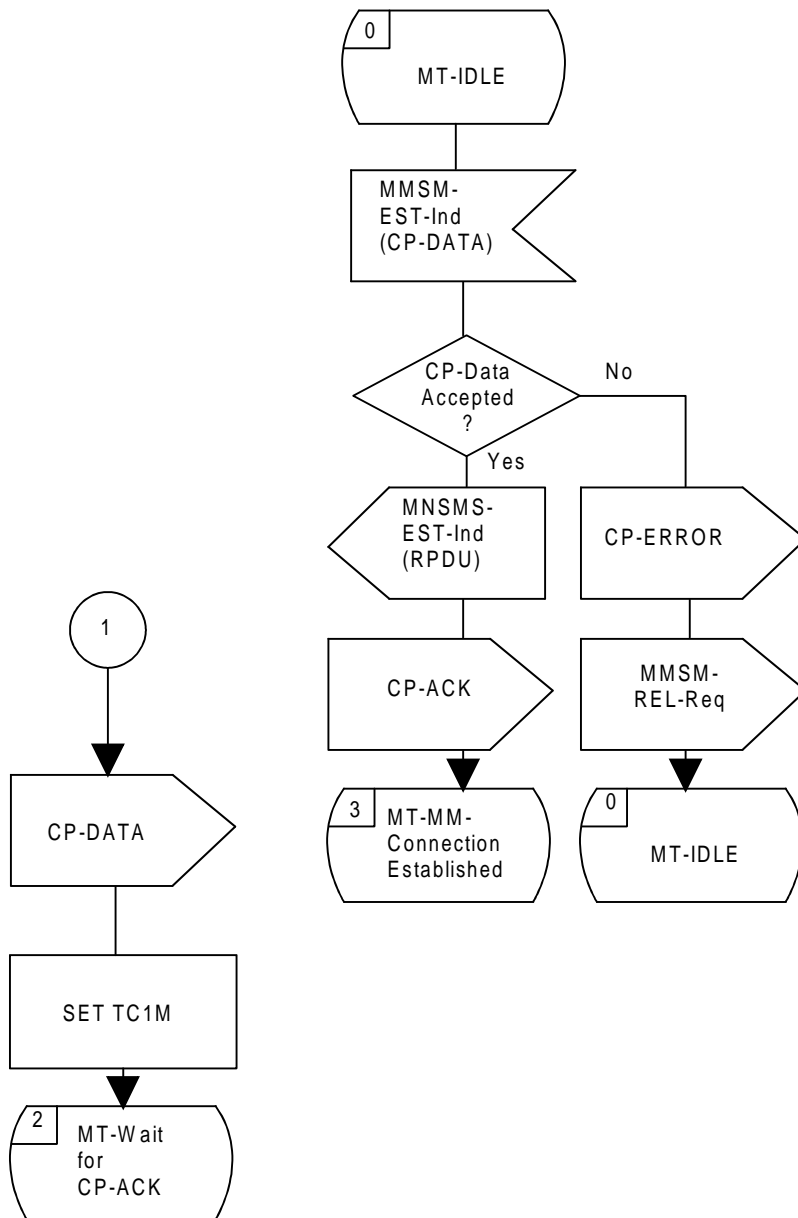
MT-SMC-entity on MS-side Initiating message transfer SDL-4
