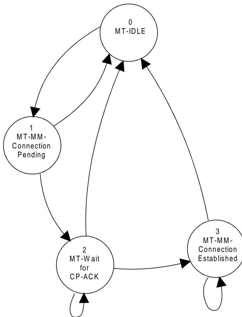
MT-SMC-entity on Network-side State transition diagram
