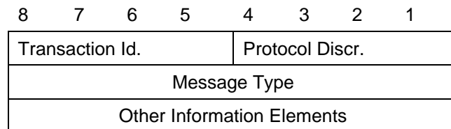
Figure 8.1/GSM 04.11
