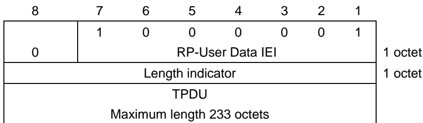
Figure 8.7/GSM 04.11: RP-User data element layout
