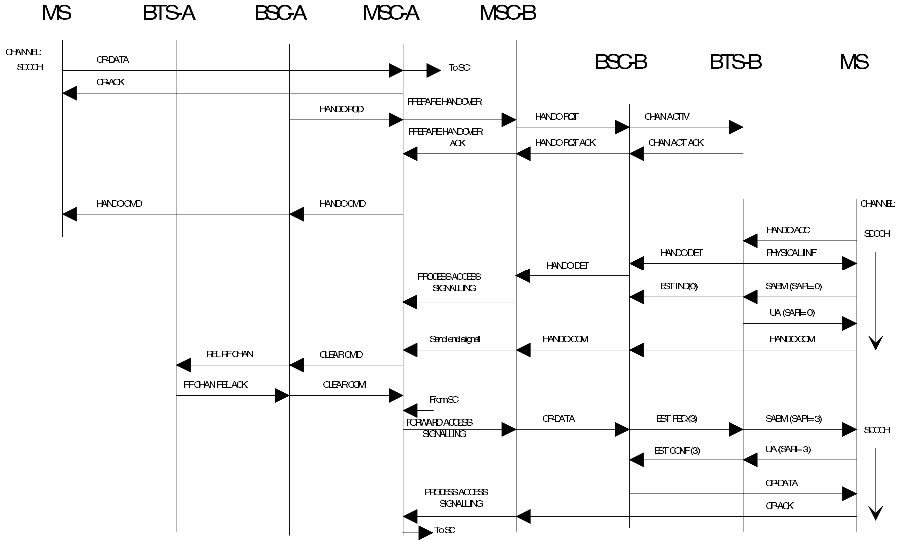
Figure F6/GSM 04.11 Inter/MS handover during Short Message transfer on SDCCH
