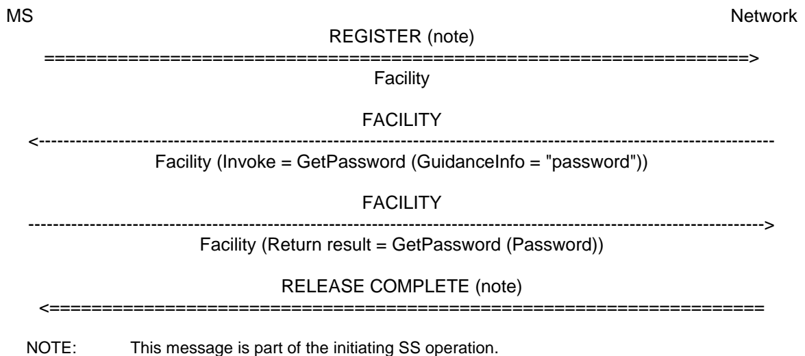
Figure 4.1: Password check: successful procedure
