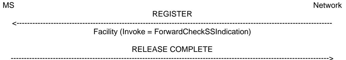
Figure 6.1: ForwardCheckSSIndication sent on new transaction
