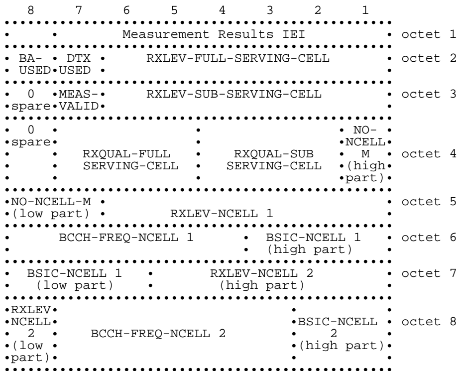
Figure 10.38/GSM 04.08 Measurement Results information element
