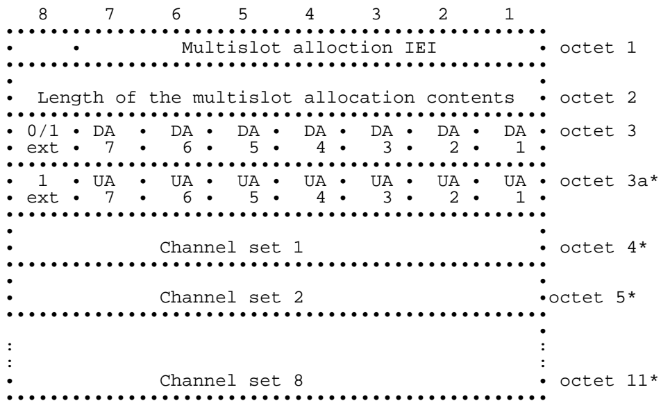
Figure 10.39b /GSM 04.08 Multislot Allocation information element
