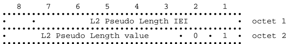
Figure 10.37/GSM 04.08 L2 Pseudo Length information element
