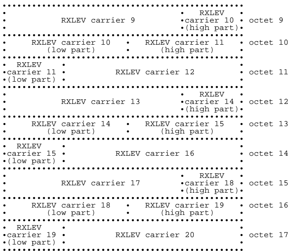
Figure 10.5.2.45.1/GSM 04.08 Extended Measurement Results information element
