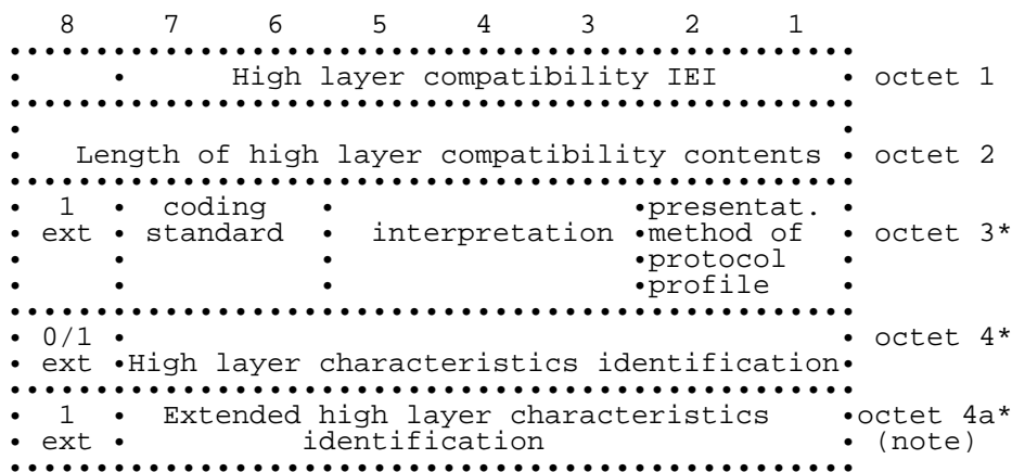
Figure 10.83/GSM 04.08 High layer compatibility information element
