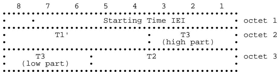
Figure 10.55/GSM 04.08: Starting Time information element
