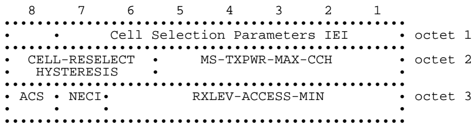
Figure 10.18/GSM 04.08: Cell Selection Parameters information element
