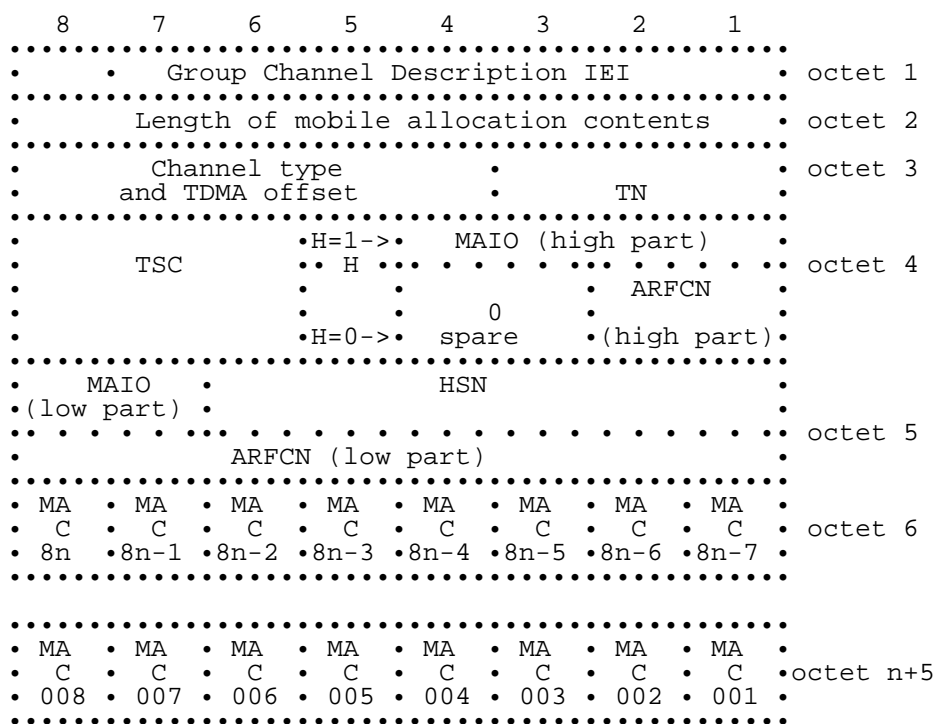
Figure 10.32a/GSM 04.08: Group Channel Description information element
