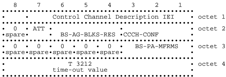
Figure 10.25/GSM 04.08: Control Channel Description information element
