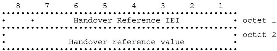
Figure 10.33/GSM 04.08: Handover Reference information element
