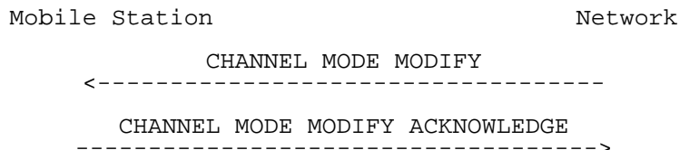
Figure 7.7/GSM 04.08: Channel mode change
