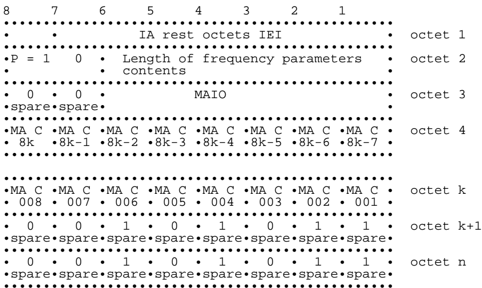
Figure 10.34a/GSM 04.08: IA Rest Octets information element, P=10
