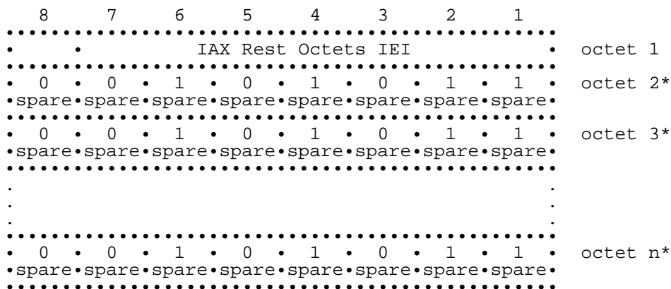
Figure 10.36/GSM 04.08: IAX Rest Octets information element
