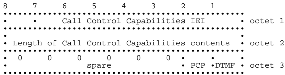
Figure 10.71a/GSM 04.08: Call Control Capabilities information element
