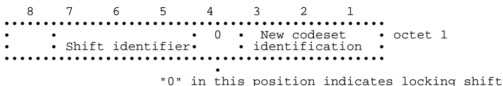
Figure 10.68/GSM 04.08: Locking shift element
