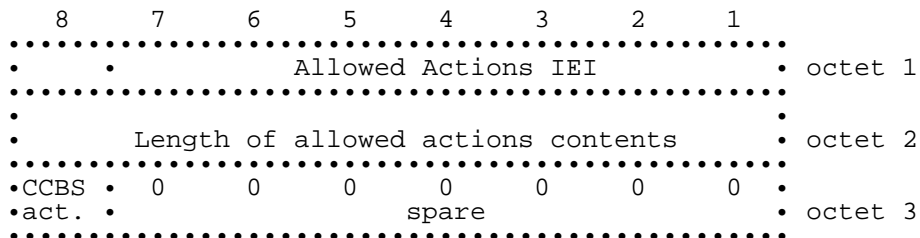
Figure 10.94/GSM 04.08: Allowed actions information element
