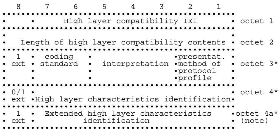
Figure 10.83/GSM 04.08: High layer compatibility information element
