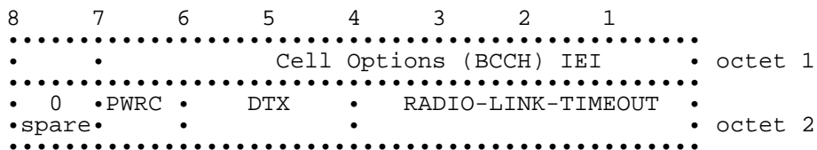
Figure 10.17/GSM 04.08: Cell Options (BCCH) information element
