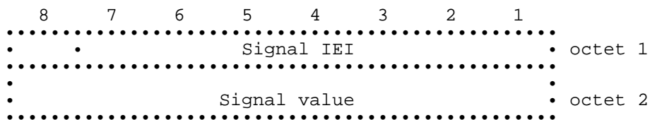
Figure 10.90/GSM 04.08: Signal information element
