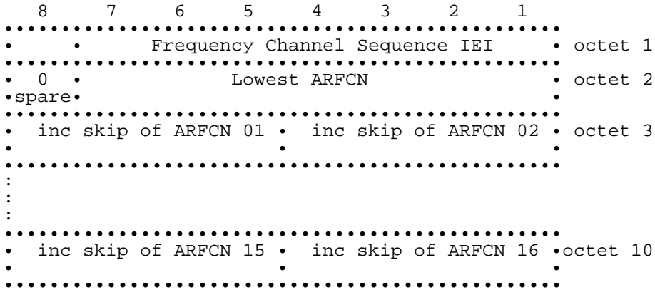
Figure 10.26/GSM 04.08: Frequency Channel Sequence information element
