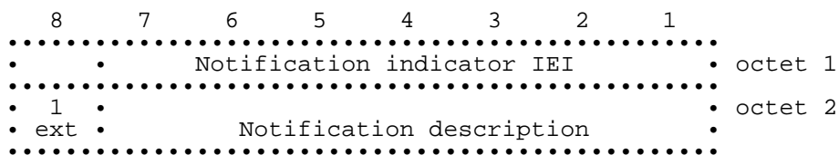
Figure 10.87/GSM 04.08: Notification indicator information element
