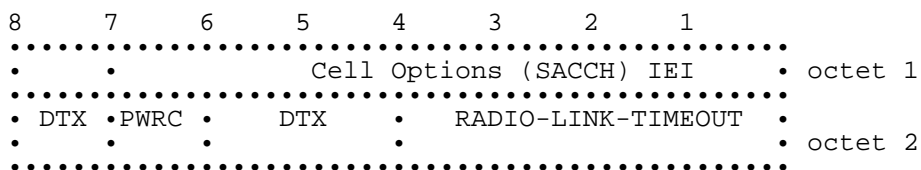
Figure 10.17a/GSM 04.08: Cell Options (SACCH) information element
