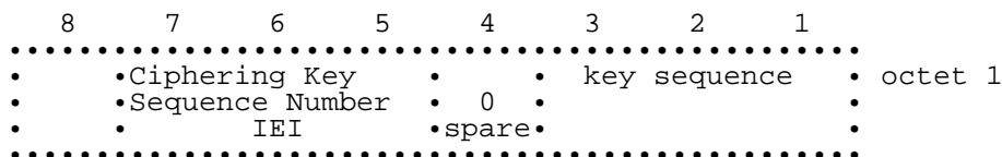
Figure 10.3/GSM 04.08: Cipherring Key Sequence Number information element
