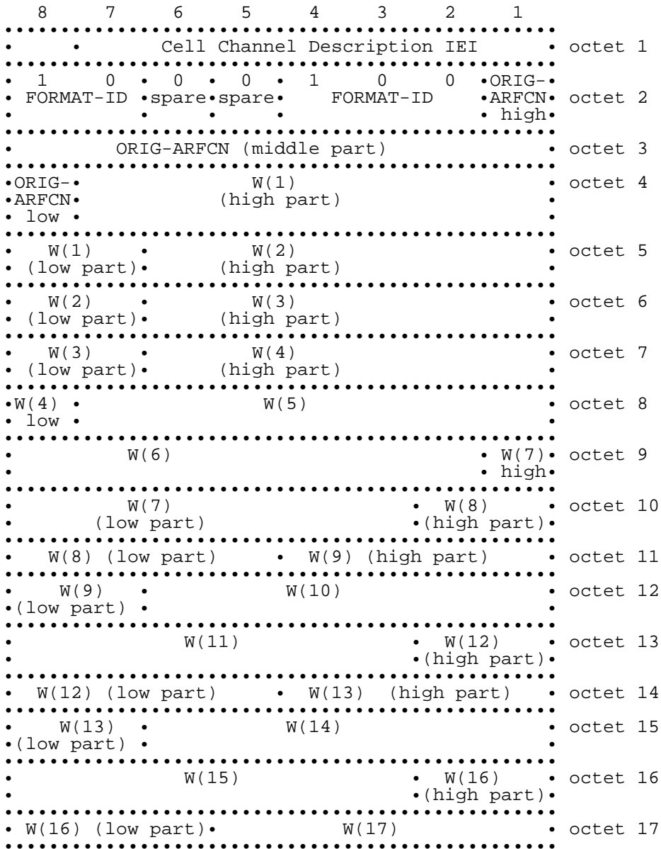
Figure 10.12/GSM 04.08: Cell Channel Description information element (512 range format)
