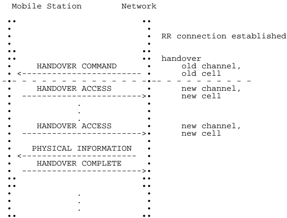
Figure 7.15/GSM 04.08: Handover to a non-synchronized cell, successful case
