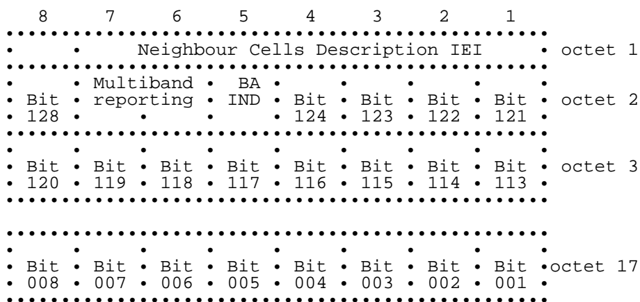
Figure 10.41/GSM 04.08: Neighbour Cells Description 2 information element
