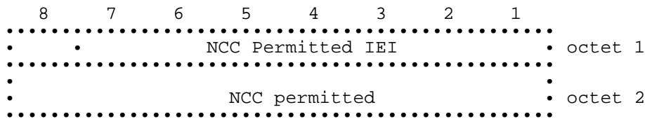
Figure 10.45/GSM 04.08: NCC Permitted information element
