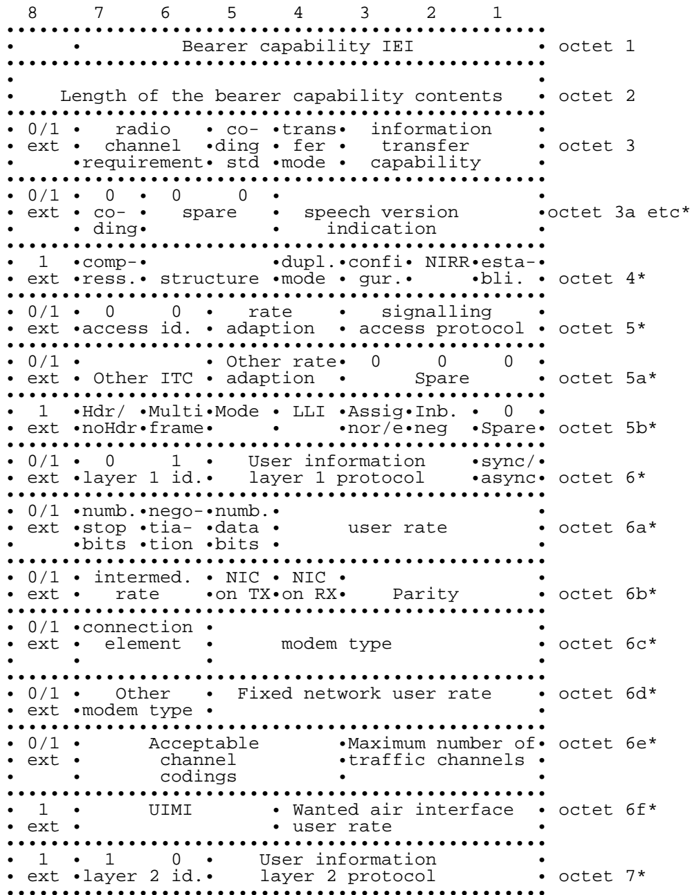
Figure 10.71/GSM 04.08: Bearer capability information element
