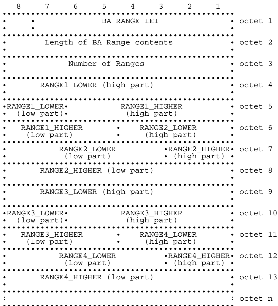
Figure 10.8a/GSM 04.08: BA RANGE information element
