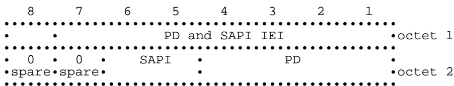
Figure 10.8qua/GSM 04.08: PD and SAPI information element
