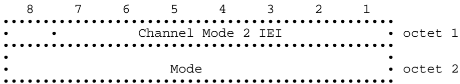
Figure 10.21/GSM 04.08: Channel Mode 2 information element
