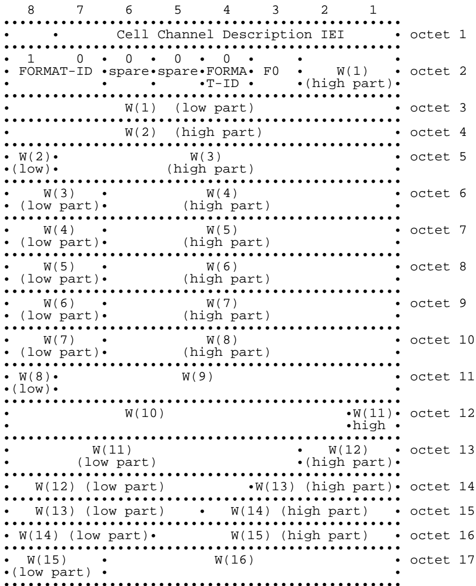
Figure 10.11/GSM 04.08: Cell Channel Description information element (1024 range format)
