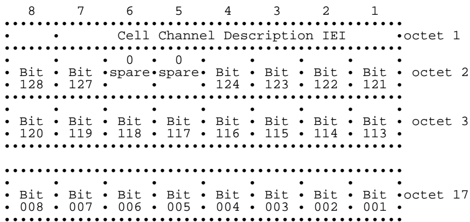
Figure 10.9/GSM 04.08: Cell Channel Description information element (general format)
