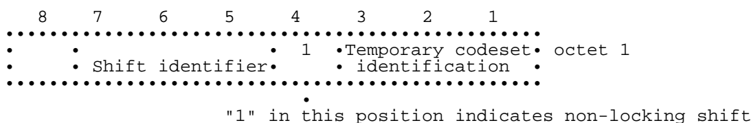
Figure 10.69/GSM 04.08: Non-locking shift element
