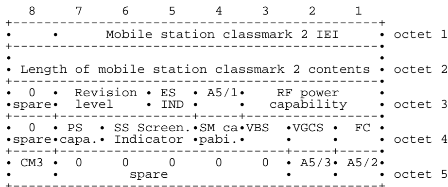
Figure 10.7/GSM 04.08: Mobile Station Classmark 2 information element
