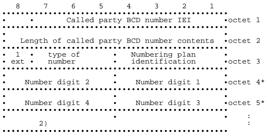
Figure 10.73/GSM 04.08: Called party BCD number information element
