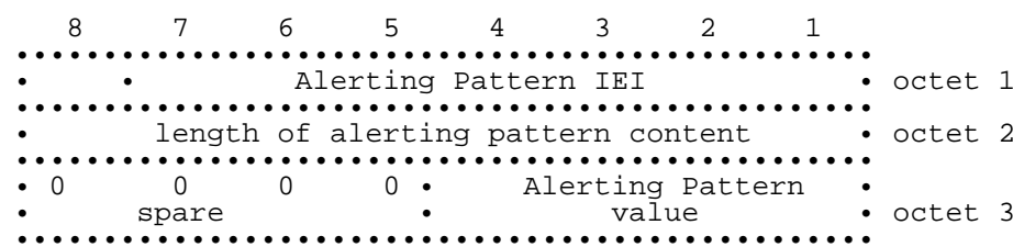
Figure 10.93/GSM 04.08: Alerting Pattern information element
