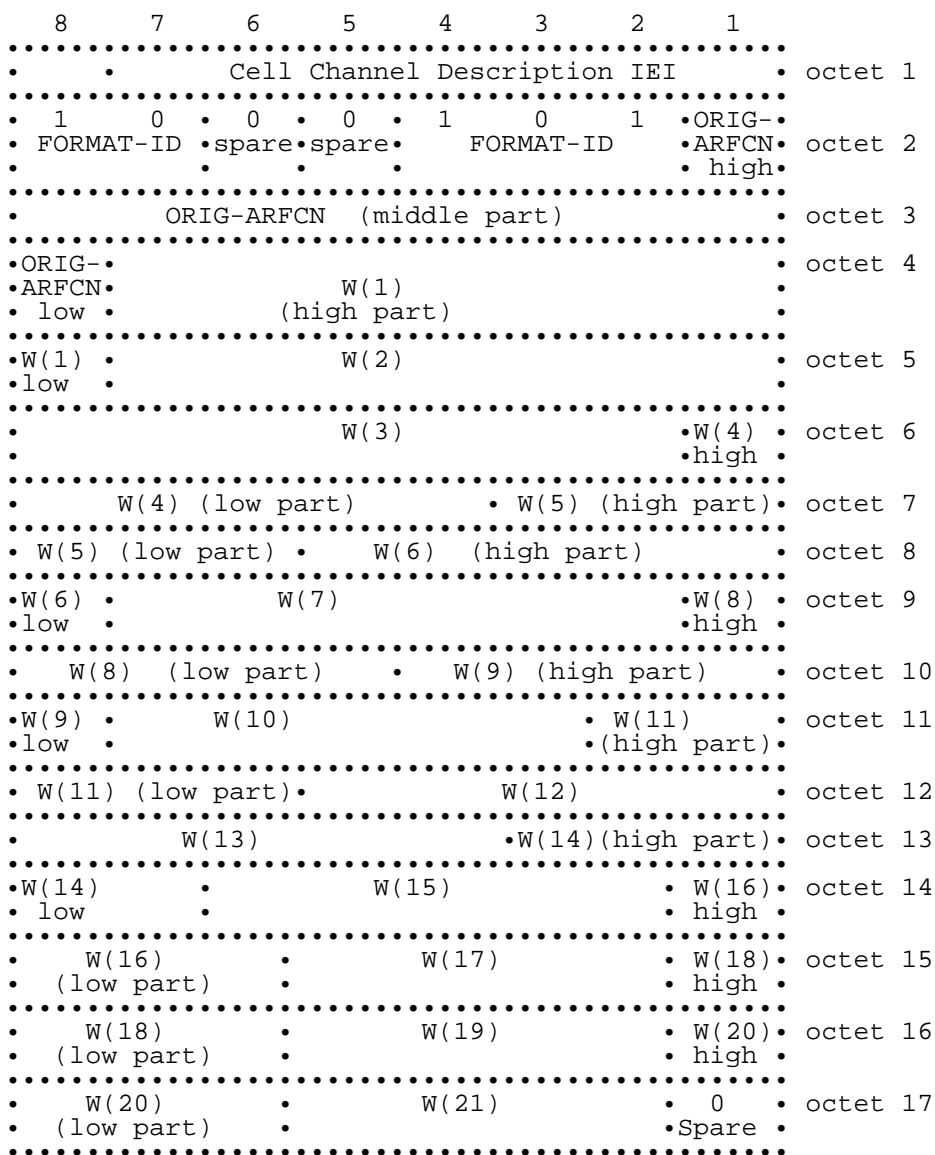
Figure 10.13/GSM 04.08: Cell Channel Description information element, range 256 format
