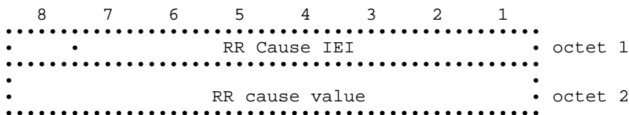
Figure 10.49/GSM 04.08: RR Cause information element
