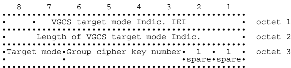
Figure 10.59c/GSM 04.08: VGCS target mode Indication information element
