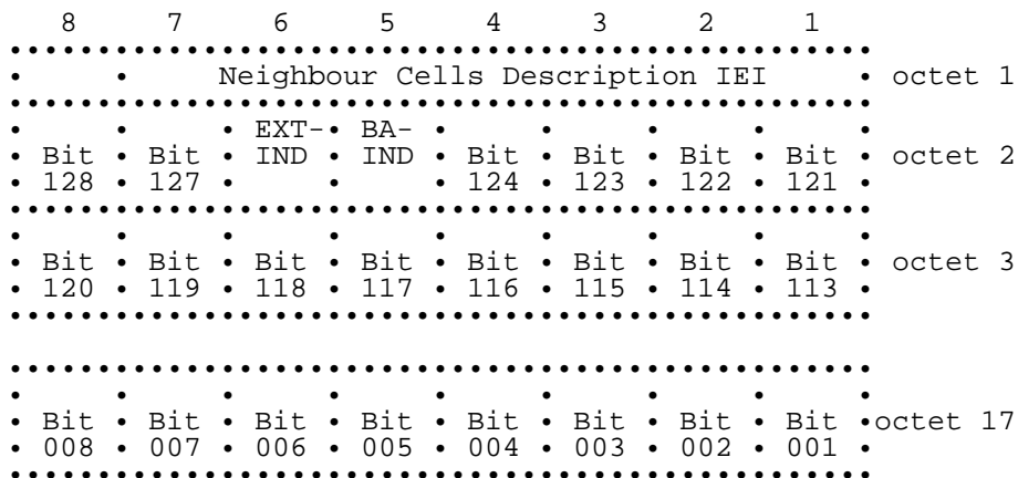
Figure 10.40/GSM 04.08: Neighbour Cells Description information element
