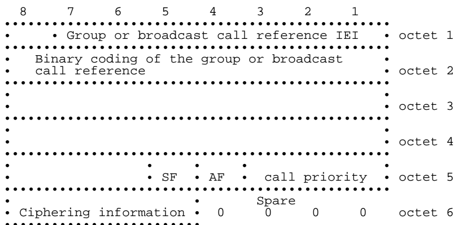
Figure 10.8bis/GSM 04.08: Descriptive Group or Broadcast Call Reference
