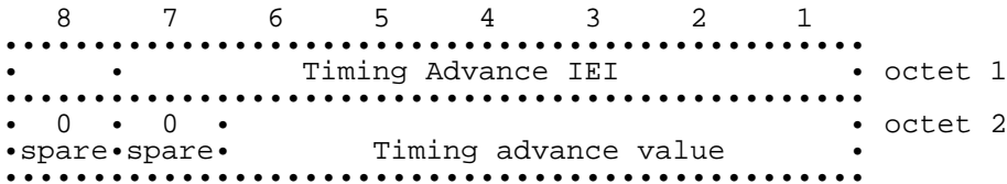
Figure 10.57/GSM 04.08: Timing Advance information element
