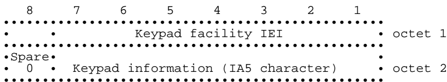
Figure 10.84/GSM 04.08: Keypad facility information element
