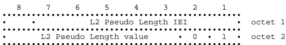
Figure 10.37/GSM 04.08: L2 Pseudo Length information element
