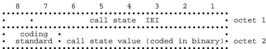
Figure 10.72/GSM 04.08: Call state information element
