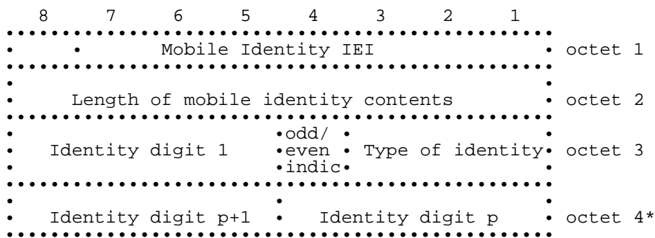
Figure 10.5/GSM 04.08: Mobile Identity information element
