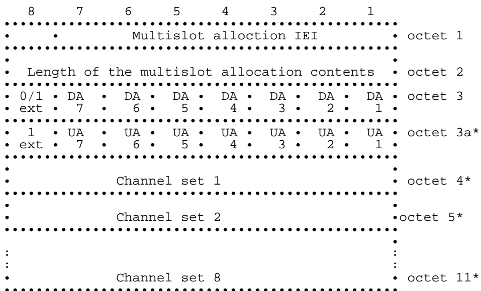
Figure 10.39b /GSM 04.08: Multislot Allocation information element
