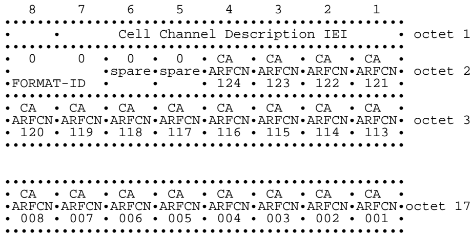
Figure 10.10/GSM 04.08: Cell Channel Description information element, bit map 0 format
