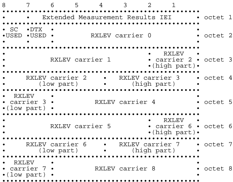
Figure 10.5.2.45.1/GSM 04.08: Extended Measurement Results information element
