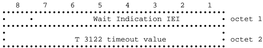
Figure 10.60/GSM 04.08: Wait Indication information element
