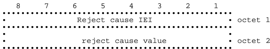
Figure 10.66/GSM 04.08: Reject Cause information element
