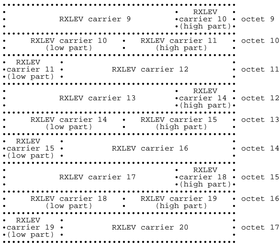
Figure 10.5.2.45.1/GSM 04.08: Extended Measurement Results information element
