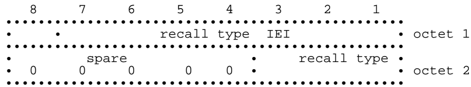
Figure 10.88a/GSM 04.08: Recall type information element
