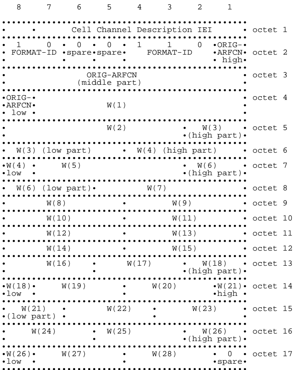
Figure 10.14/GSM 04.08: Cell Channel Description information element, range 128 format
