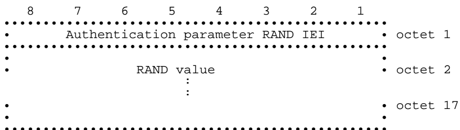
Figure 10.61/GSM 04.08: Authentication Parameter RAND information element
