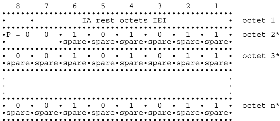
Figure 10.34/GSM 04.08: IA rest octets information element, P=00
