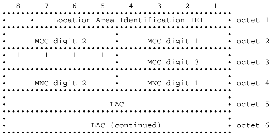
Figure 10.4/GSM 04.08: Location Area Identification information element
