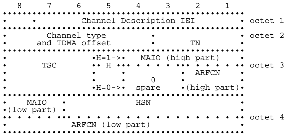
Figure 10.19a/GSM 04.08: Channel Description 2 information element
