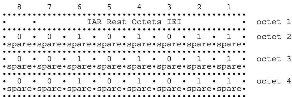
Figure 10.35/GSM 04.08: IAR Rest Octets information element
