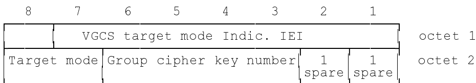
Figure 10.59c/GSM 04.08 VGCS target mode Indication information element
