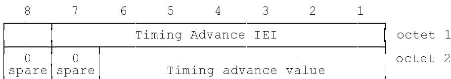
Figure 10.57/GSM 04.08 Timing Advance information element
