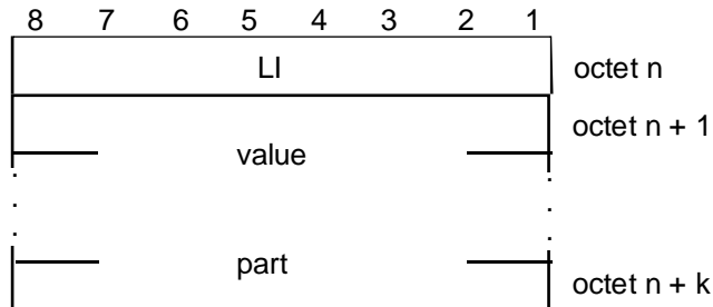
Figure 11.7/GSM 04.07 Type 4 IE of format LV (k = 0, 1, 2, ...)
