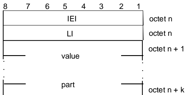
Figure 11.8/GSM 04.07 Type 4 IE of format TLV (k = 1, 2, ...)
