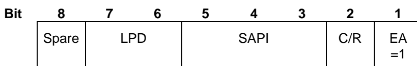
Figure 4/GSM 04.06: Address field format
