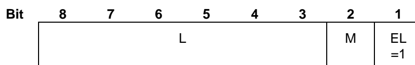
Figure 5/GSM 04.06: Length indicator field format
