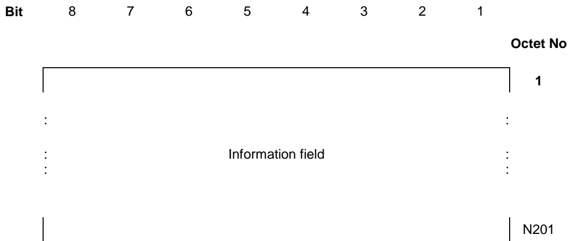
Figure 1/GSM 04.06 (sheet 2 of 3): General frame formats
