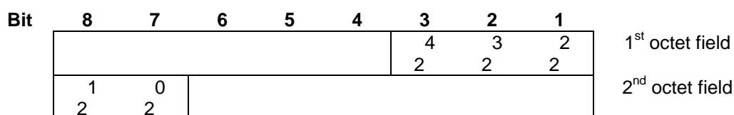
Figure 3/GSM 04.06: Field mapping convention
