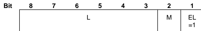
Figure 5/GSM 04.06: Length indicator field format
