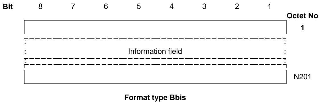
Figure 1/GSM 04.06 (sheet 2 of 3): General frame formats
