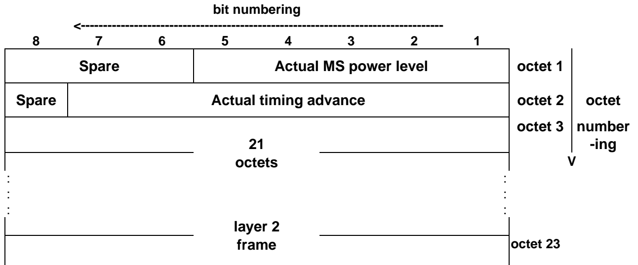
Figure 7.2: SACCH uplink block format
