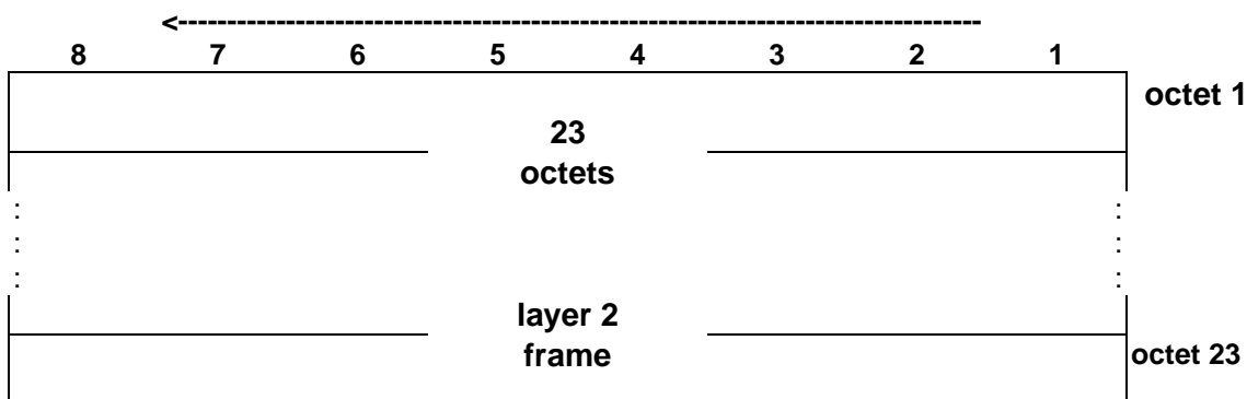
Figure 7.4: FACCH/SDCCH uplink block format
