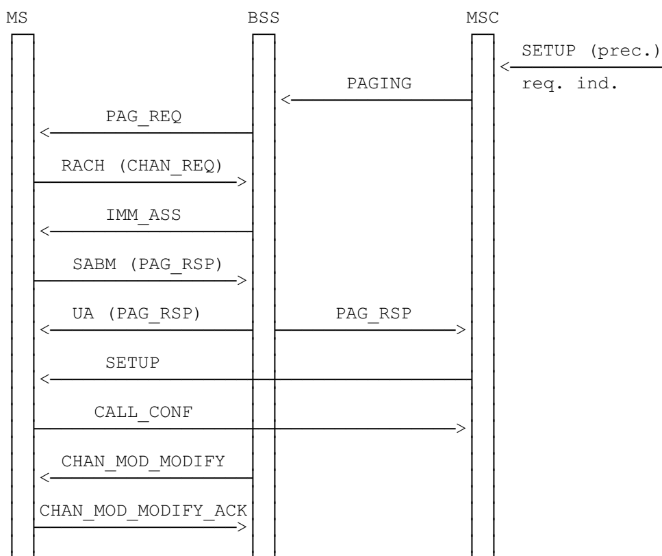
Figure 4: Signalling information required for the prioritization at mobile terminating call establishment with fast call set-up and without called-party pre-emption
