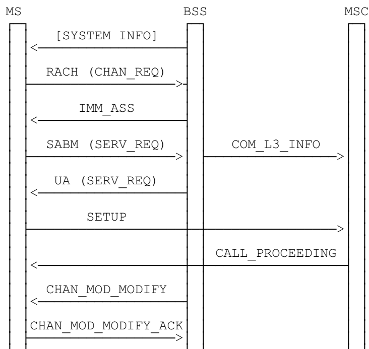
Figure 2: Signalling information required for the prioritization at mobile originating call establishment with fast call set-up
