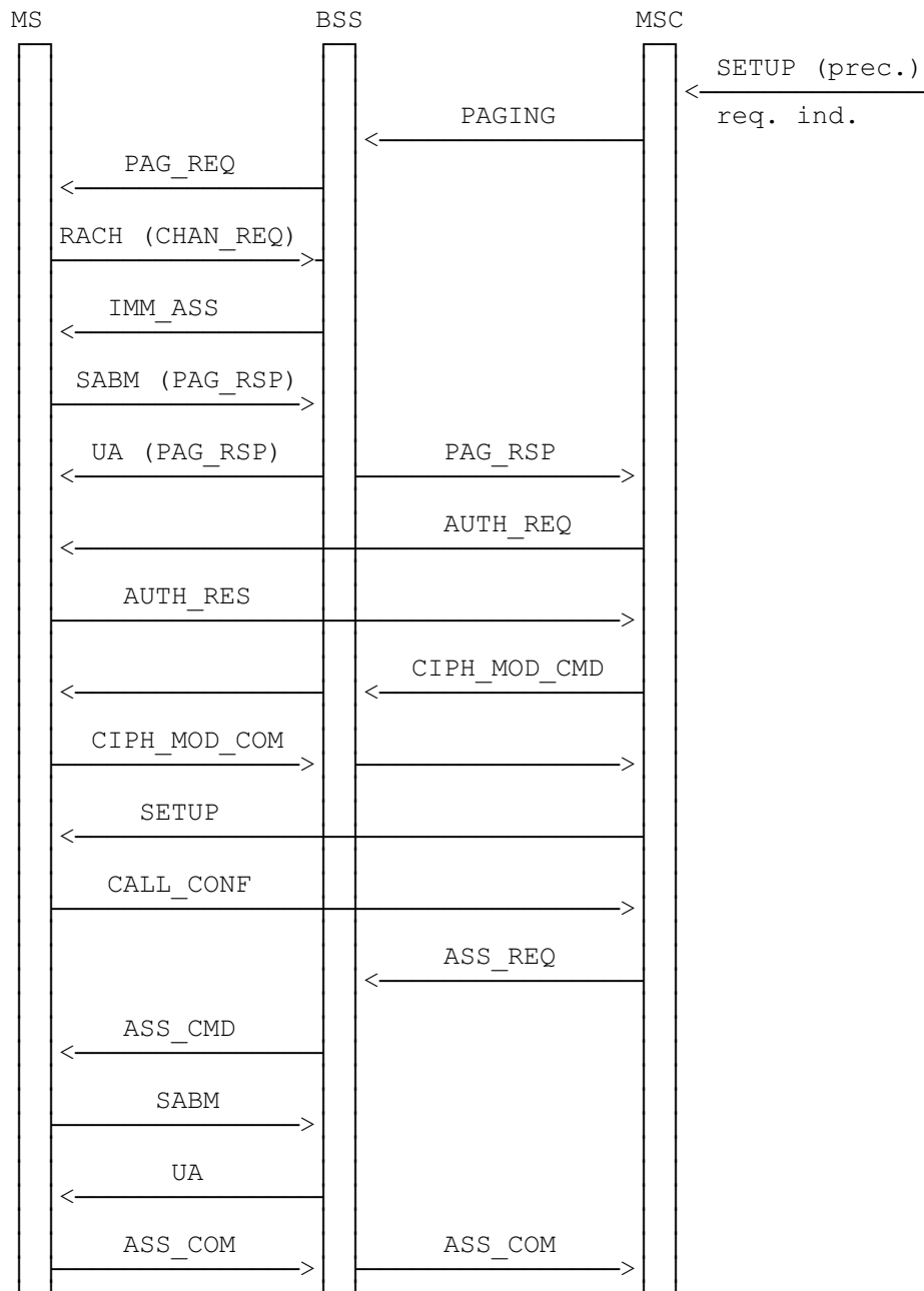
Figure 3: Signalling information required for the prioritization at mobile terminating call establishment without fast call set-up and without called-party pre-emption
