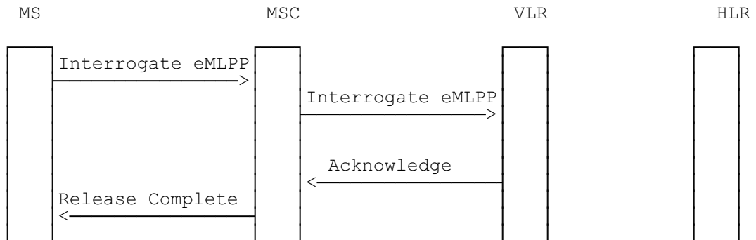
Figure 8: Interrogation of eMLPP
