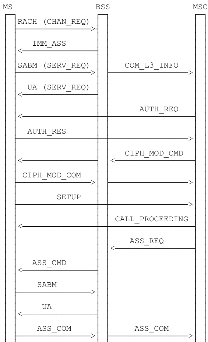
Figure 1: Signalling information required for the prioritization at mobile originating call establishment without fast call set-up
