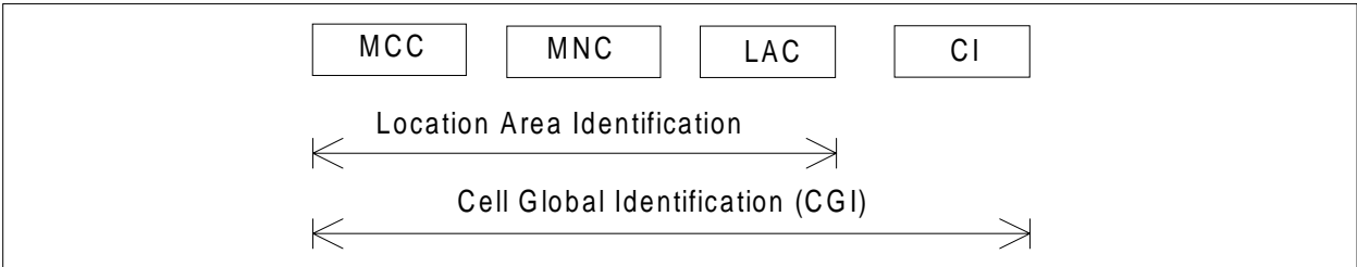
Figure 4: Structure of Cell Global Identification
