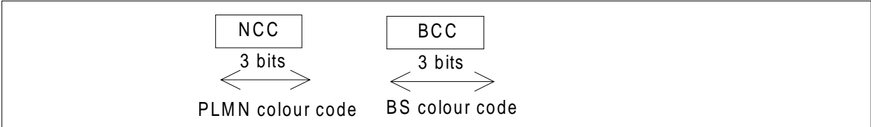
Figure 5: Structure of BSIC
