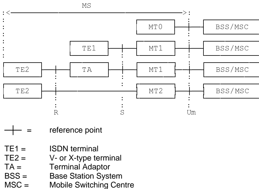
Figure 1: GSM PLMN Access Reference Configuration
