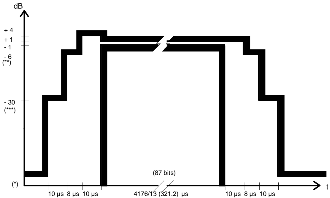
Time mask for access burst (AB)
