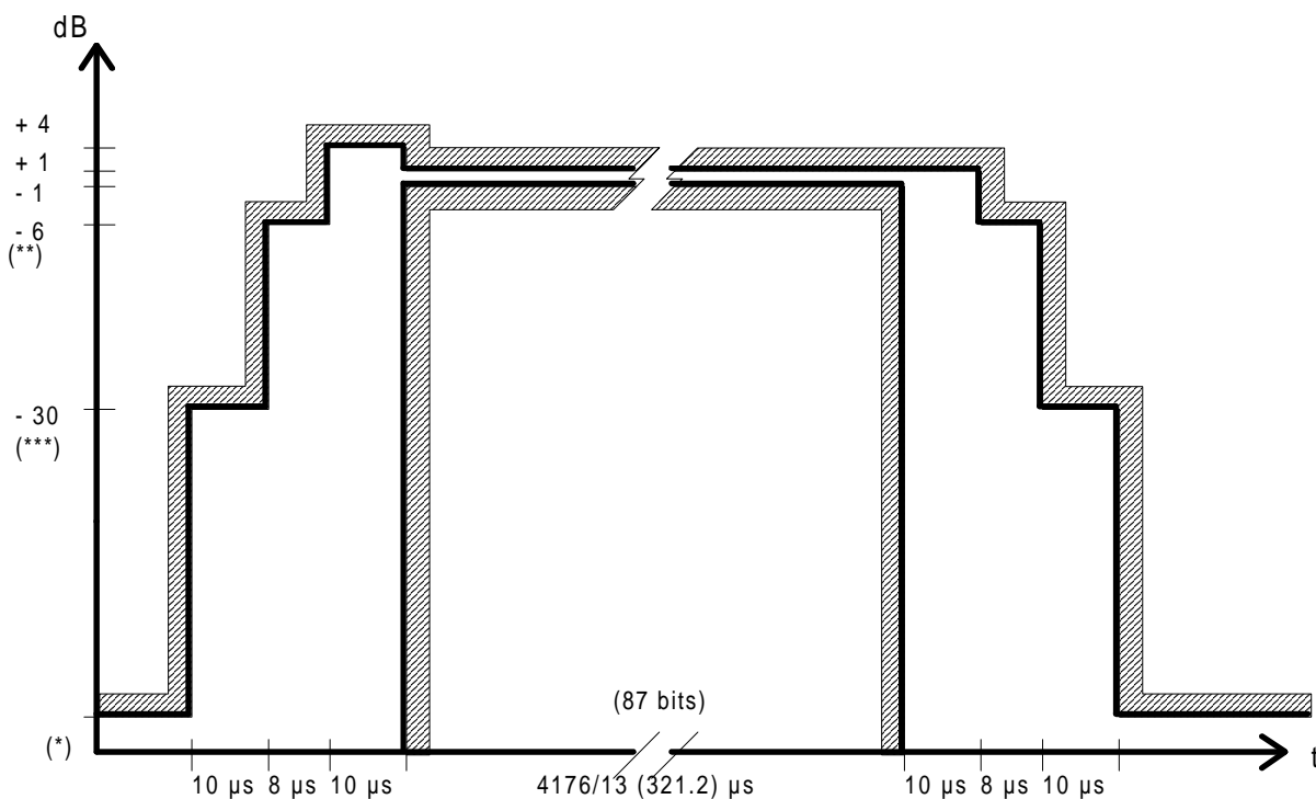
Time mask for access burst (AB)
