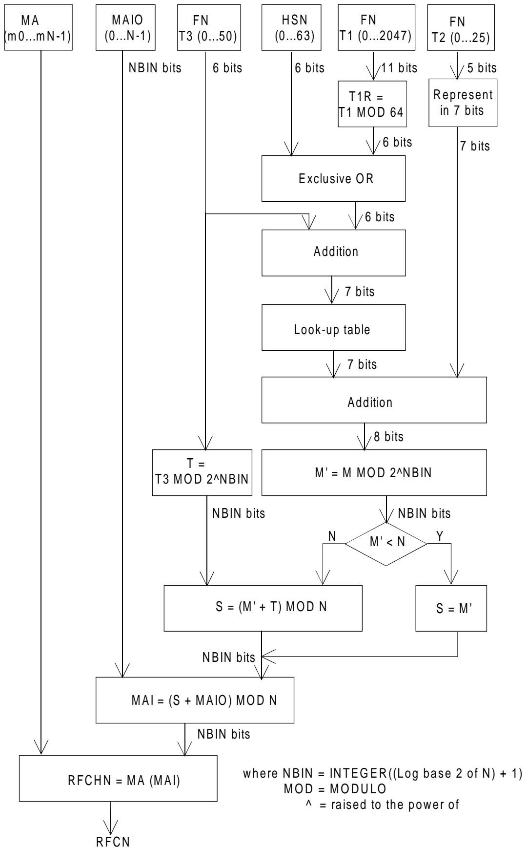
Figure 6: Block diagram of the frequency hopping algorithm when HSN ≠ 0
