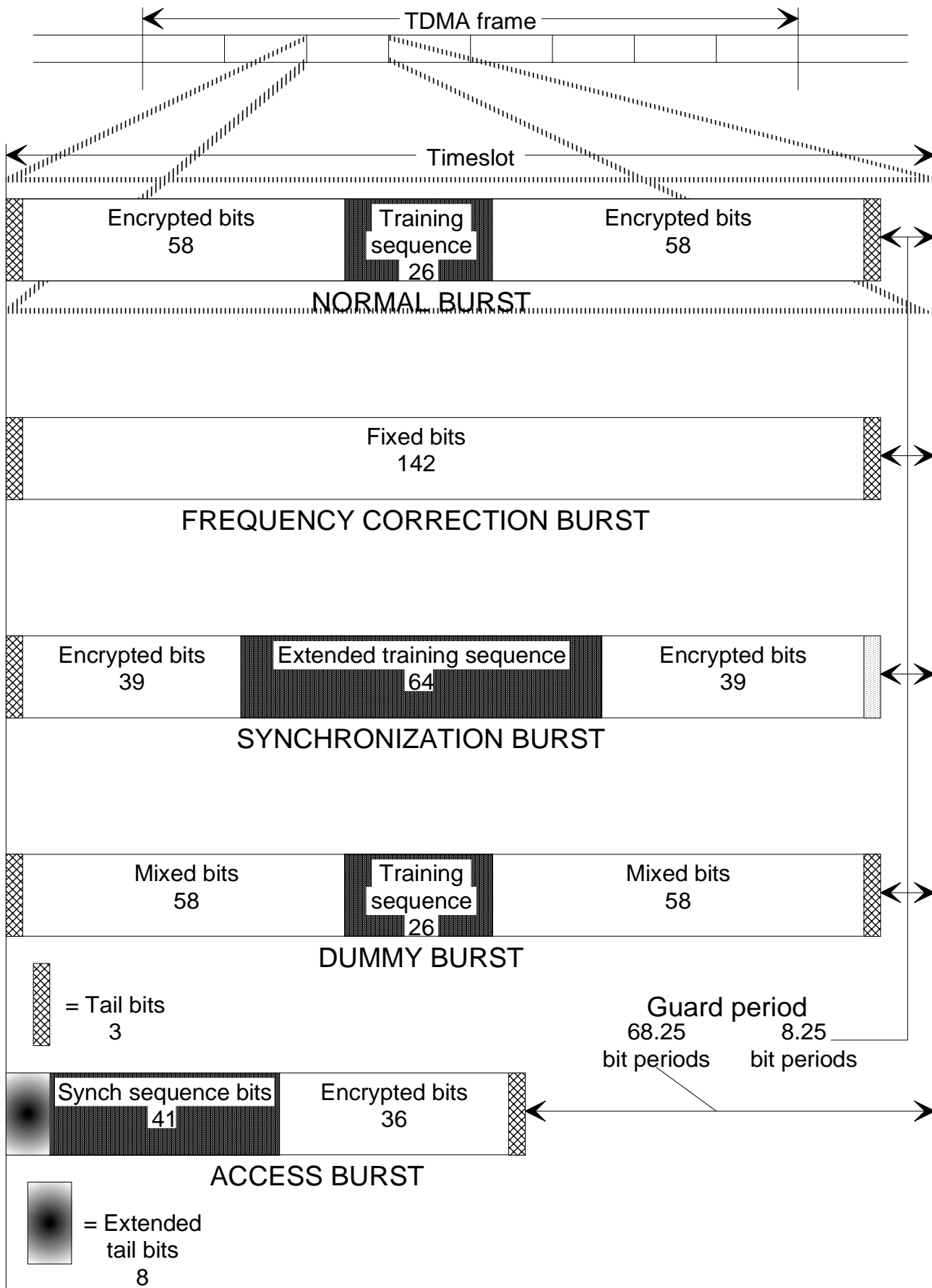
Figure 3: Timeslot and format of bursts
