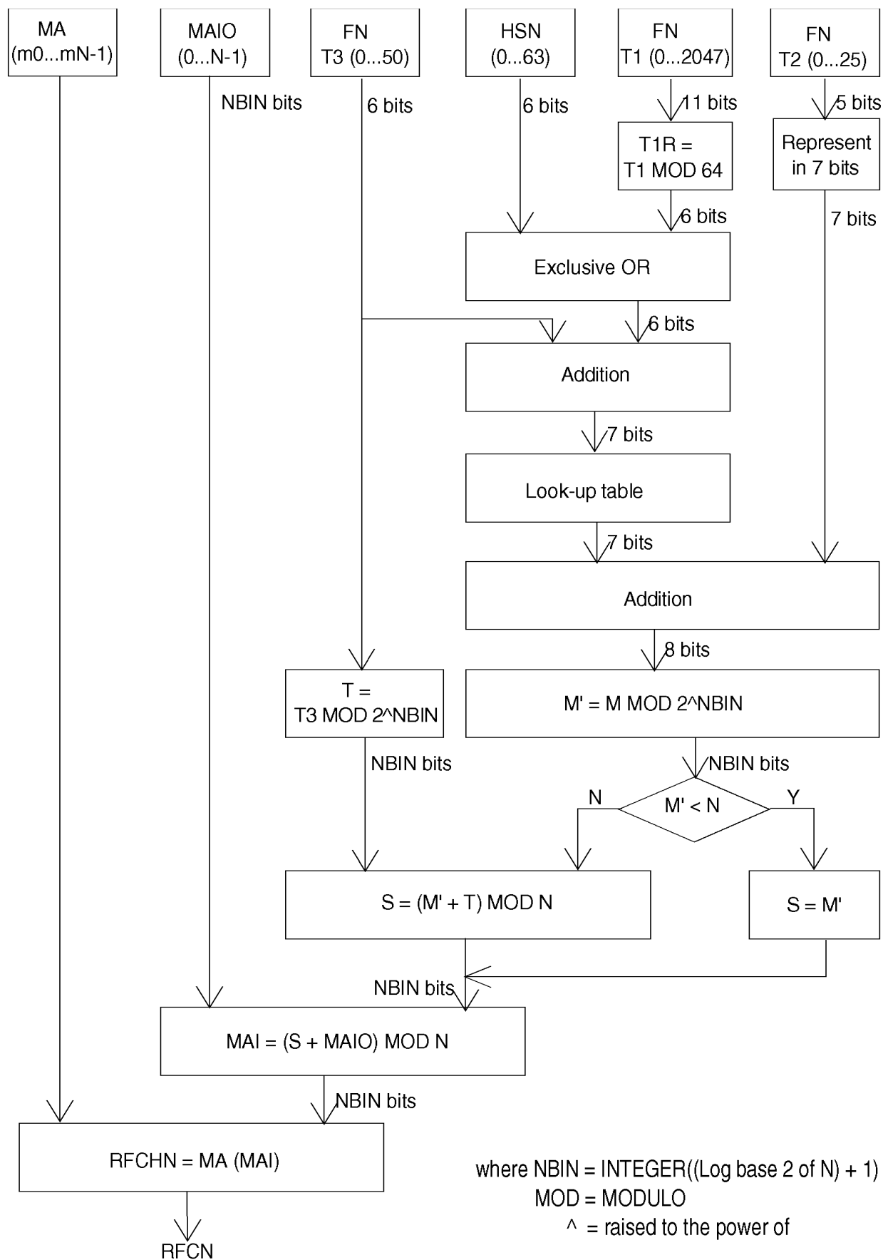
Figure 6: Block diagram of the frequency hopping algorithm when \text{HSN} \neq 0
