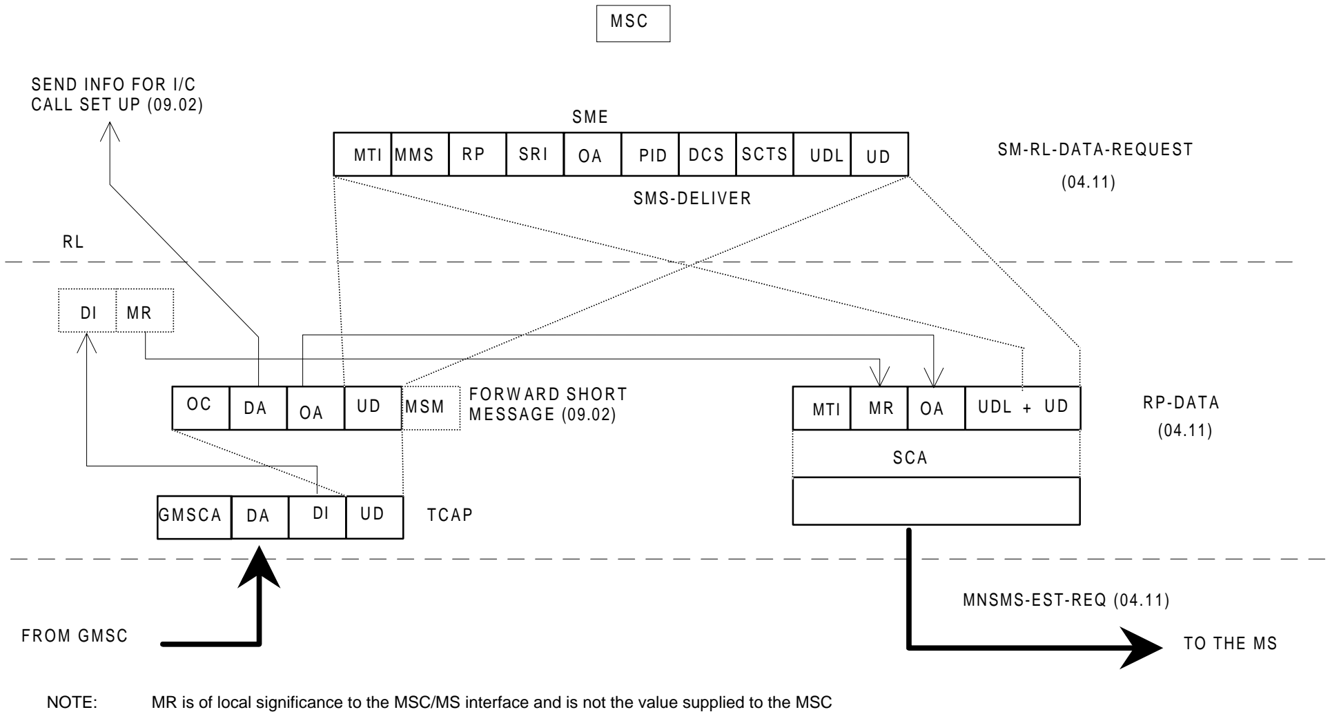
Figure 1.3: Mobile terminated short message
