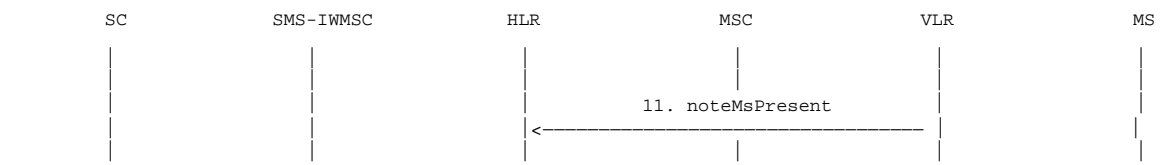
Figure 03.40/20b: The alert procedure when the MS becomes reachable, MNRF is set and MCEF is set
