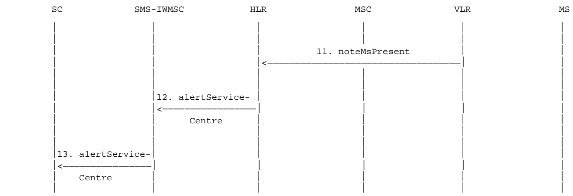
Figure 03.40/20a: The alert procedure when the MS becomes reachable, MNRF is set and MCEF is not set
