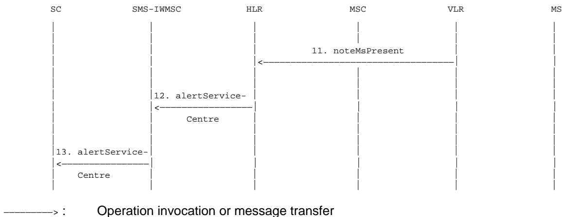
Figure 03.40/20a: The alert procedure when the MS becomes reachable, MNRF is set and MCEF is not set
