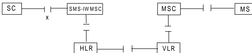
Figure 03.40/19: Interfaces involved in the Alert procedure. X is the interface between an SC and an MSC as defined in section 5
