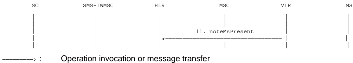
Figure 03.40/20b: The alert procedure when the MS becomes reachable, MNRF is set and MCEF is set
