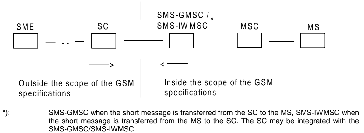
Figure 03.40/4: Entities involved in the provision of SM MT and SM MO: SC, SMS-GMSC/SMS-IWMSC, MSC and MS
