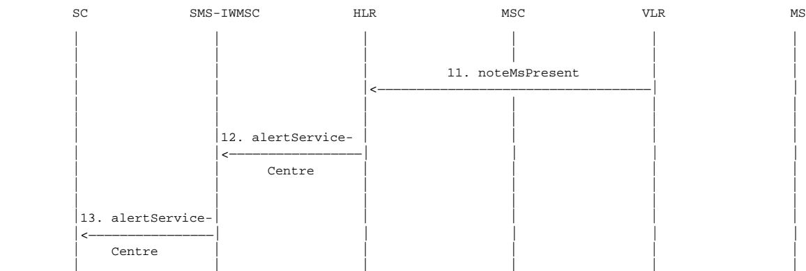
Figure 03.40/20a: The alert procedure when the MS becomes reachable, MNRF is set and MCEF is not set
