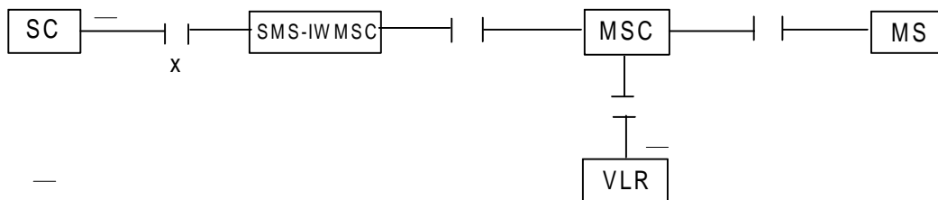
Figure 03.40/17: Interfaces involved in the Short message mobile originated procedure
