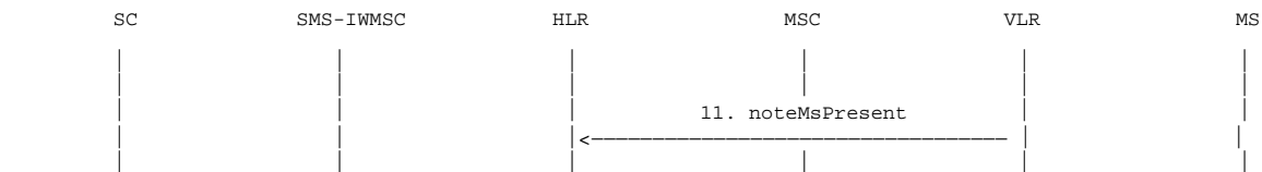
Figure 03.40/20b: The alert procedure when the MS becomes reachable, MNRF is set and MCEF is set
