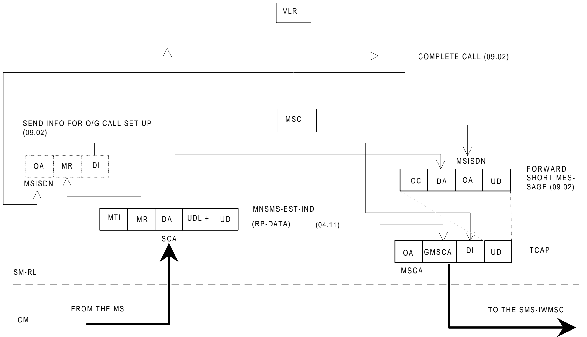
Figure 3.2: Mobile originated short message
