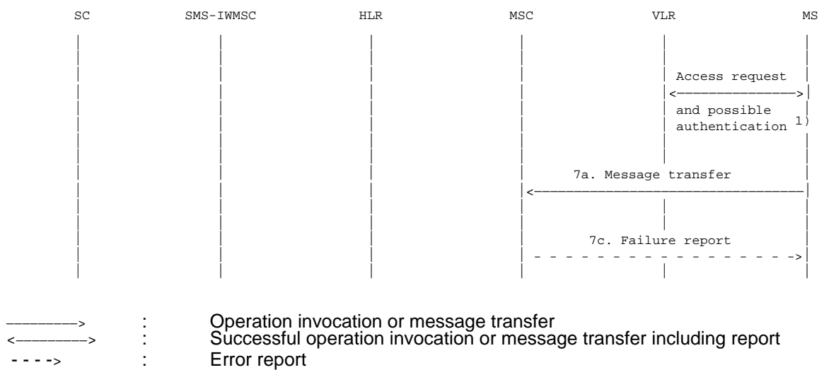
Figure 03.40/18a): Successful short message transfer attempt
