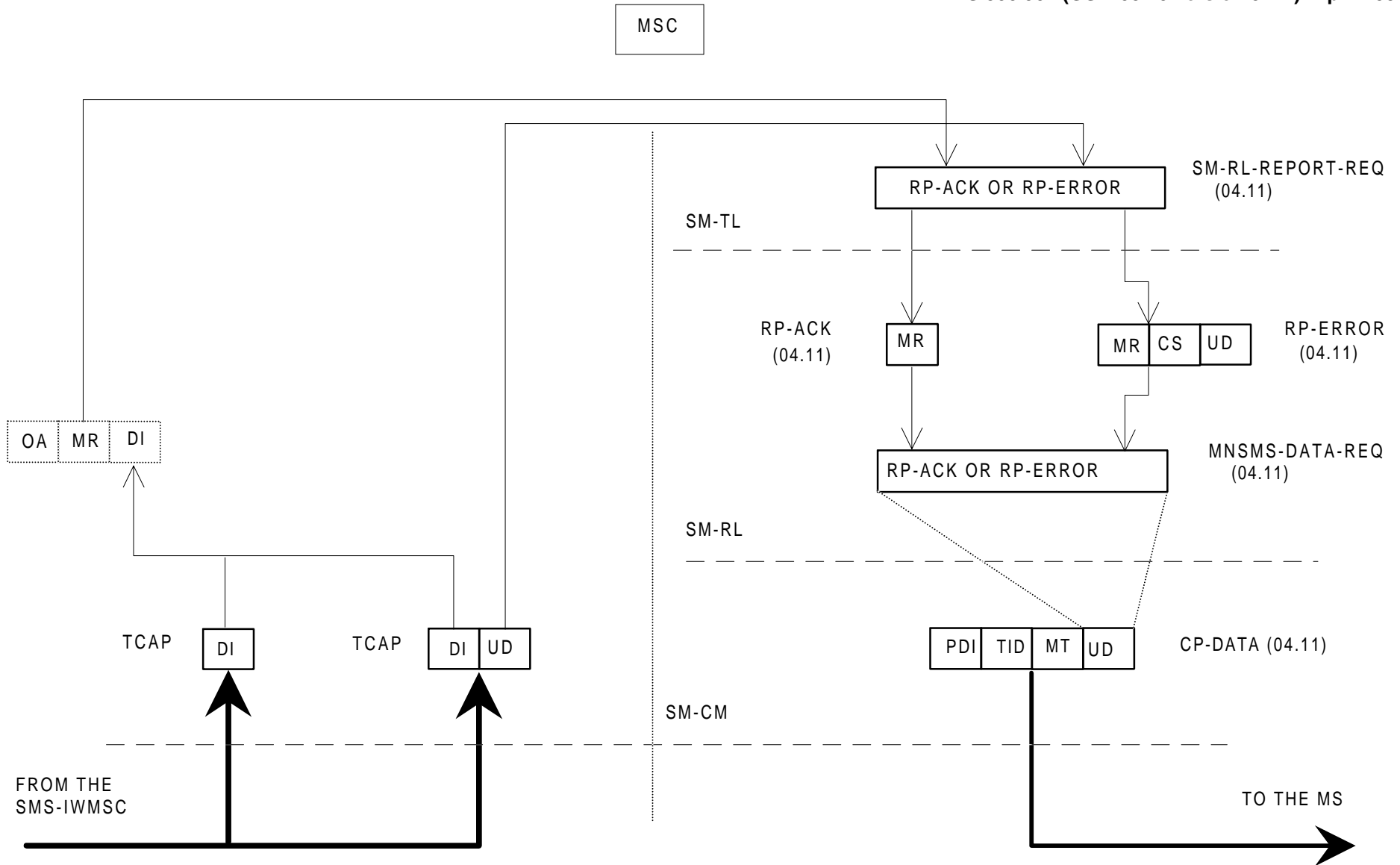
Figure 4.2: Acknowledgement in the MO case
