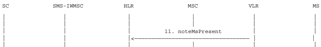
Figure 03.40/20b: The alert procedure when the MS becomes reachable, MNRF is set and MCEF is set
