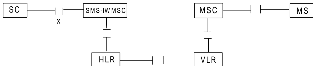
Figure 03.40/19: Interfaces involved in the Alert procedure. X is the interface between an SC and an MSC as defined in clause 5
