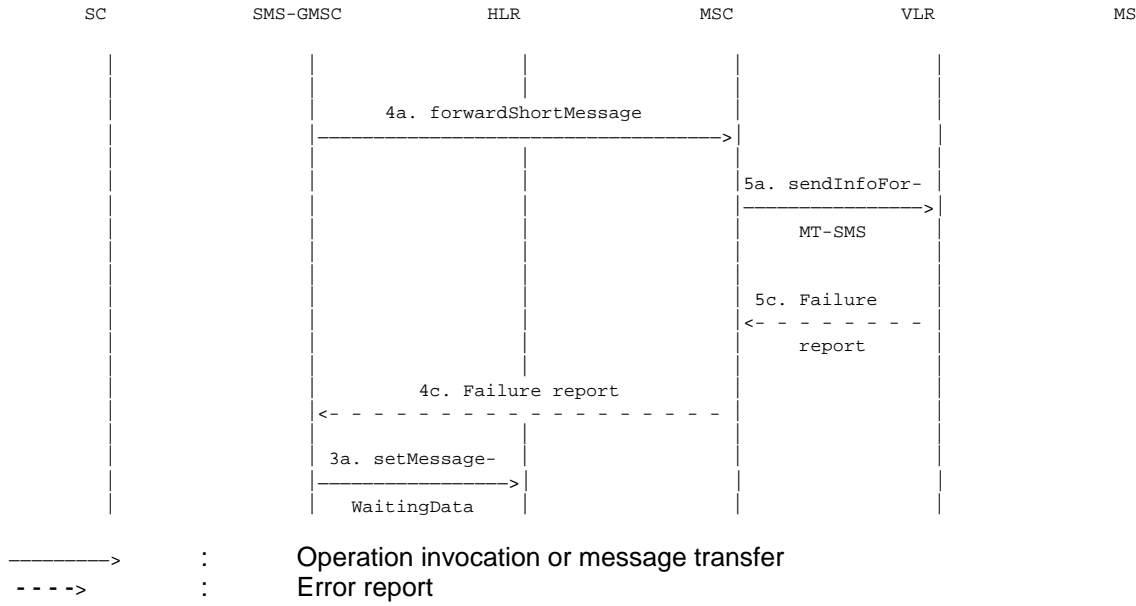
Figure 03.40/16b): "Send information for MT SMS" procedure; erroneous case: absent subscriber (e.g. IMSI DETACH)
