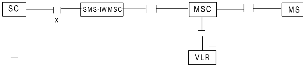
Figure 03.40/17: Interfaces involved in the Short message mobile originated procedure. GSM 03.02. X is the interface between an MSC and an SC as defined in chapter 5
