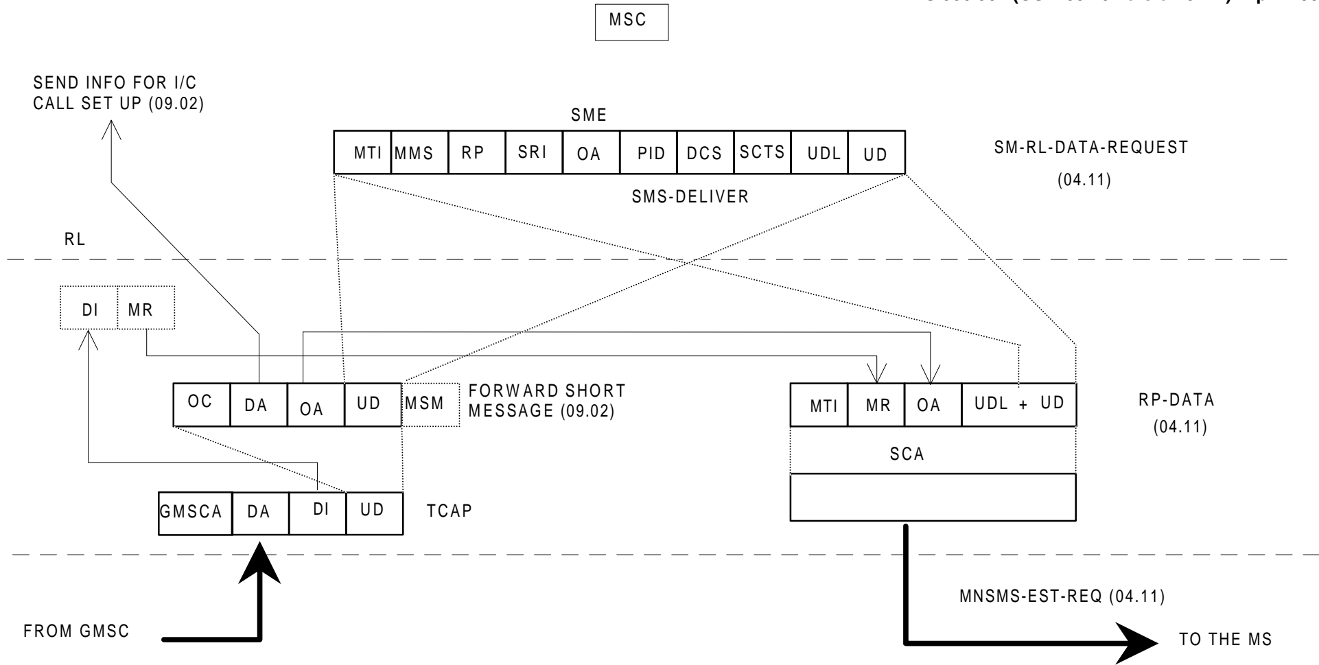
Figure 1.3: Mobile terminated short message
