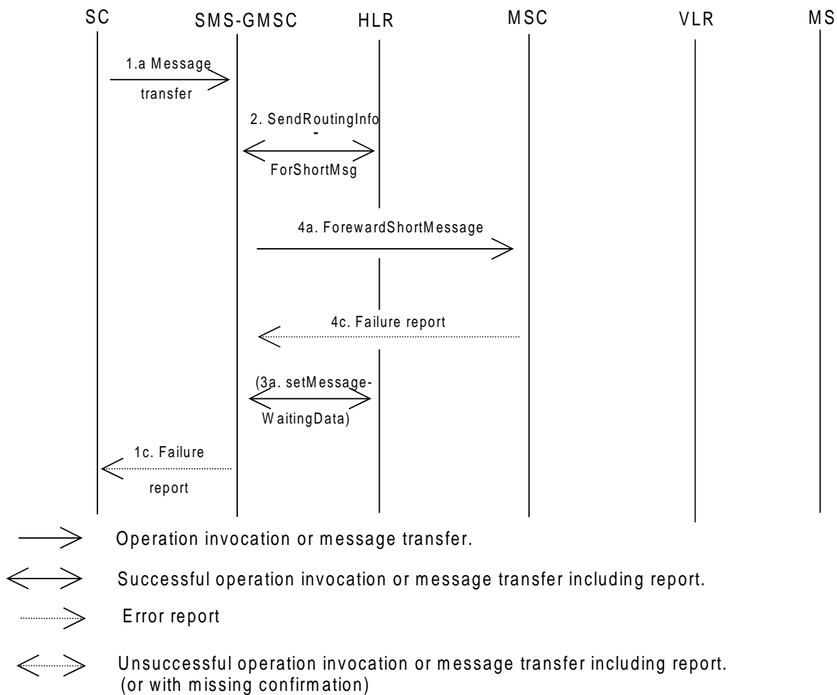
Figure 03.40/15d): Short message transfer attempt failing due to error at the MSC
