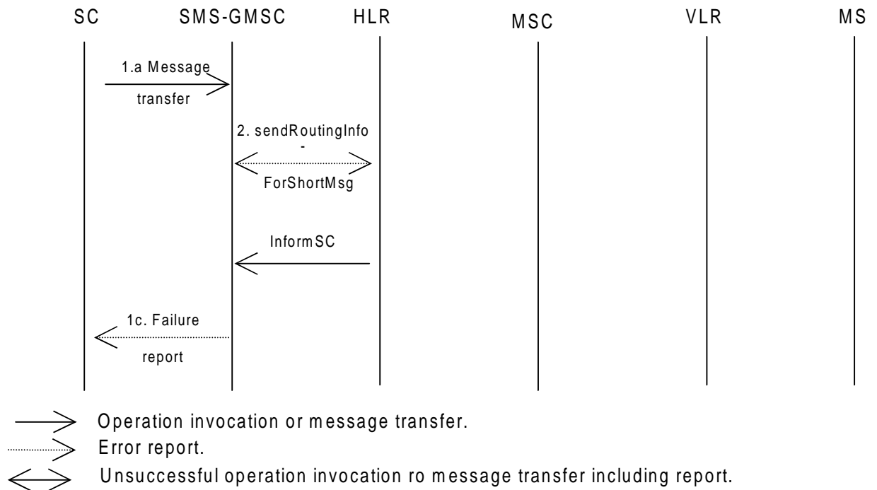
Figure 03.40/15c): Short message transfer attempt failing due to negative outcome of HLR information retrieval
