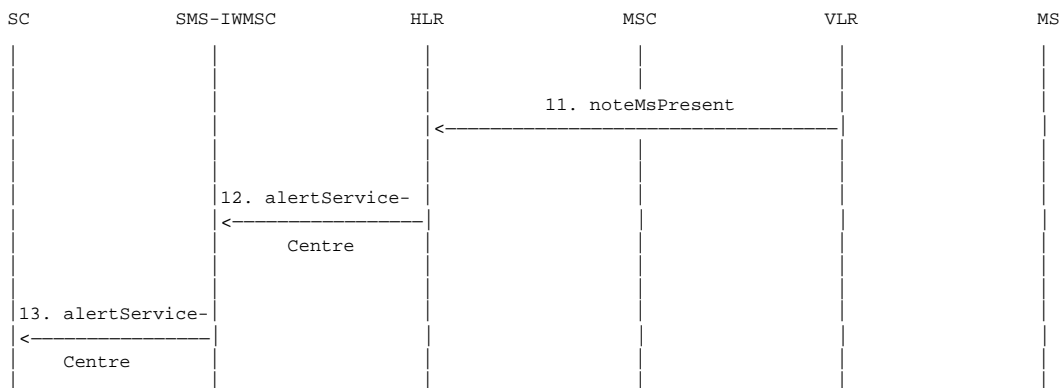
Figure 03.40/20a: The alert procedure when the MS becomes reachable, MNRF is set and MCEF is not set
