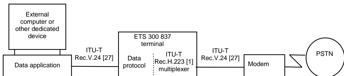
Figure 2: Data application - data protocol interface
