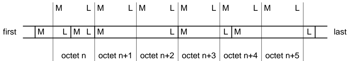
Figure C.2: Output split into bytes
