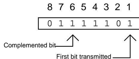
Figure B.1: Control escape byte for HDLC frame tunneling procedure
