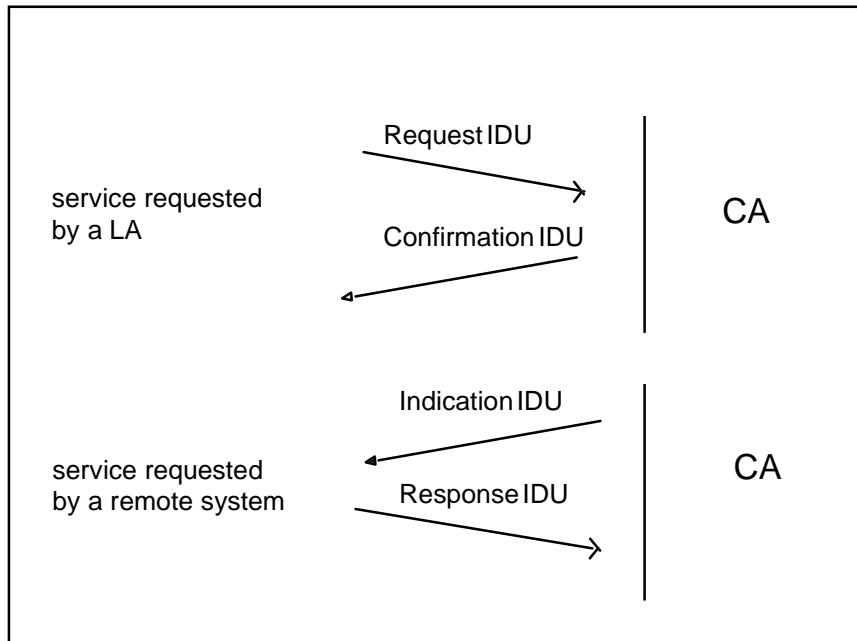
General sequence of IDUs exchanged at the PCI
