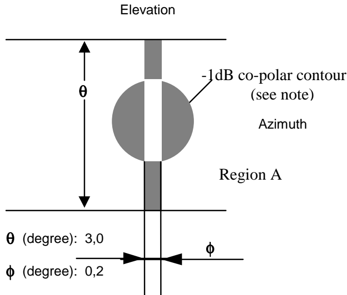
Figure 9: Mask for XPD measurements around the main beam axis
