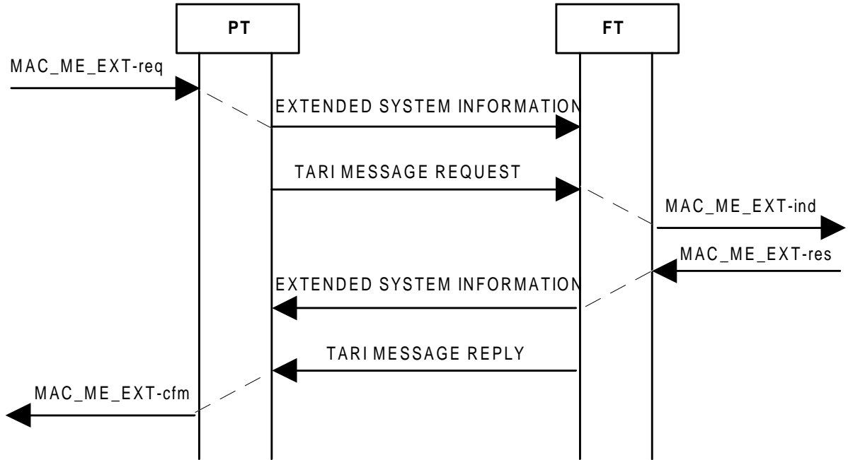
Figure 4: Non-continuous broadcast
