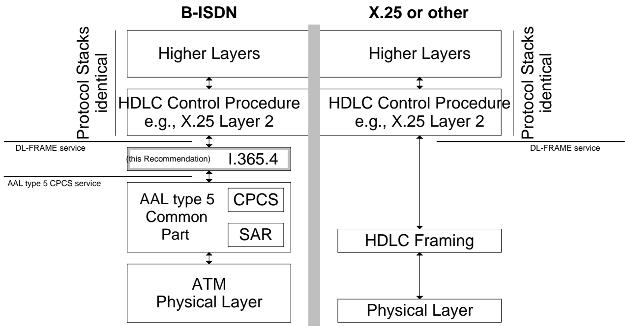
Figure 1: ITU-T Recommendation I.365.4 [5]: Environment for the DL-FRAME SSCS for HDLC Applications
