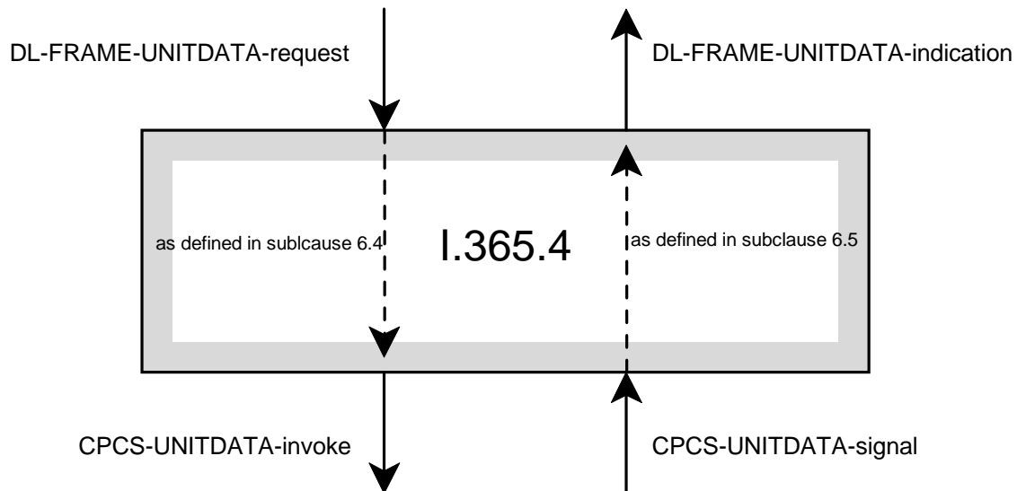
Figure 2: ITU-T Recommendation I.365.4 [5]: Relationship of DL-FRAME primitives and AAL type 5 CPCS signals
