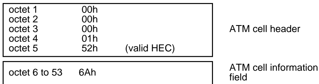
Figure 6: Cell rate decoupling
