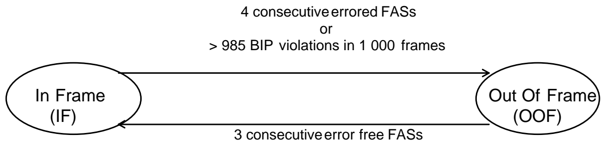
Figure 18: Frame alignment state diagram
