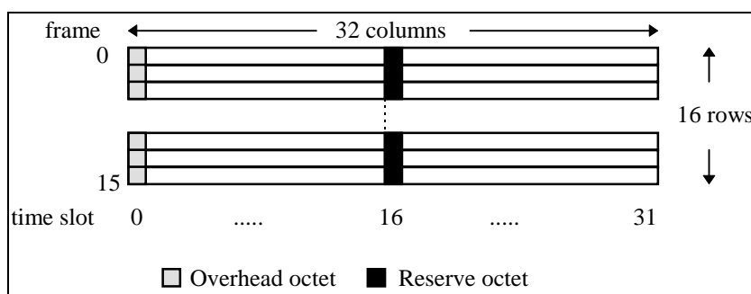
Figure 10: Multiframe at 2 048 kbit/s
