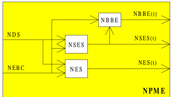
Figure 25: Near-end performance monitoring event (NPME) function
