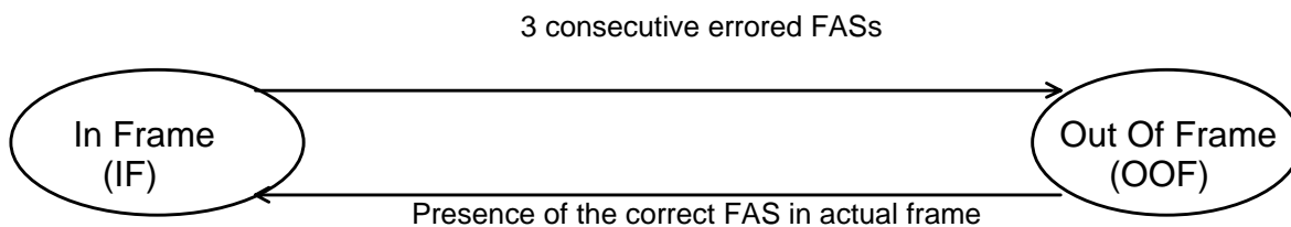
Figure 15: Frame alignment state diagram
