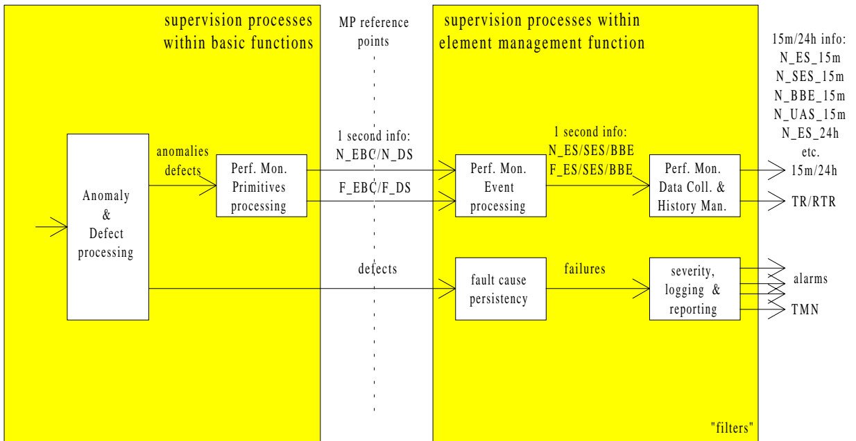
Figure 24: Supervision process within equipment management function
