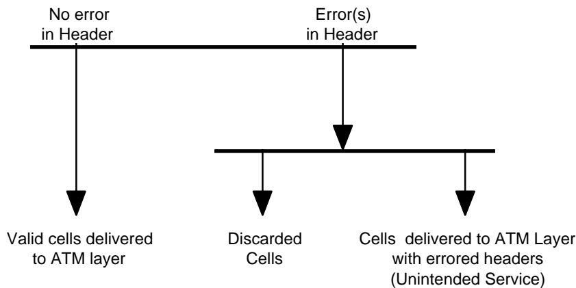
Figure13: HEC verification flow
