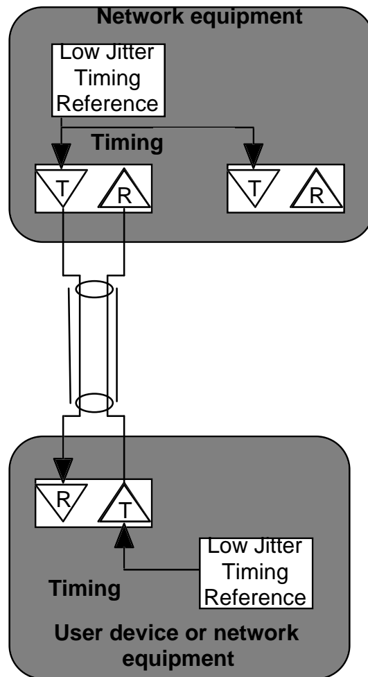
Figure 3: User device—network equipment timing configurations
