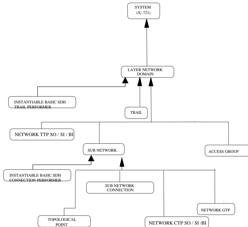
Figure 14: Naming diagram
