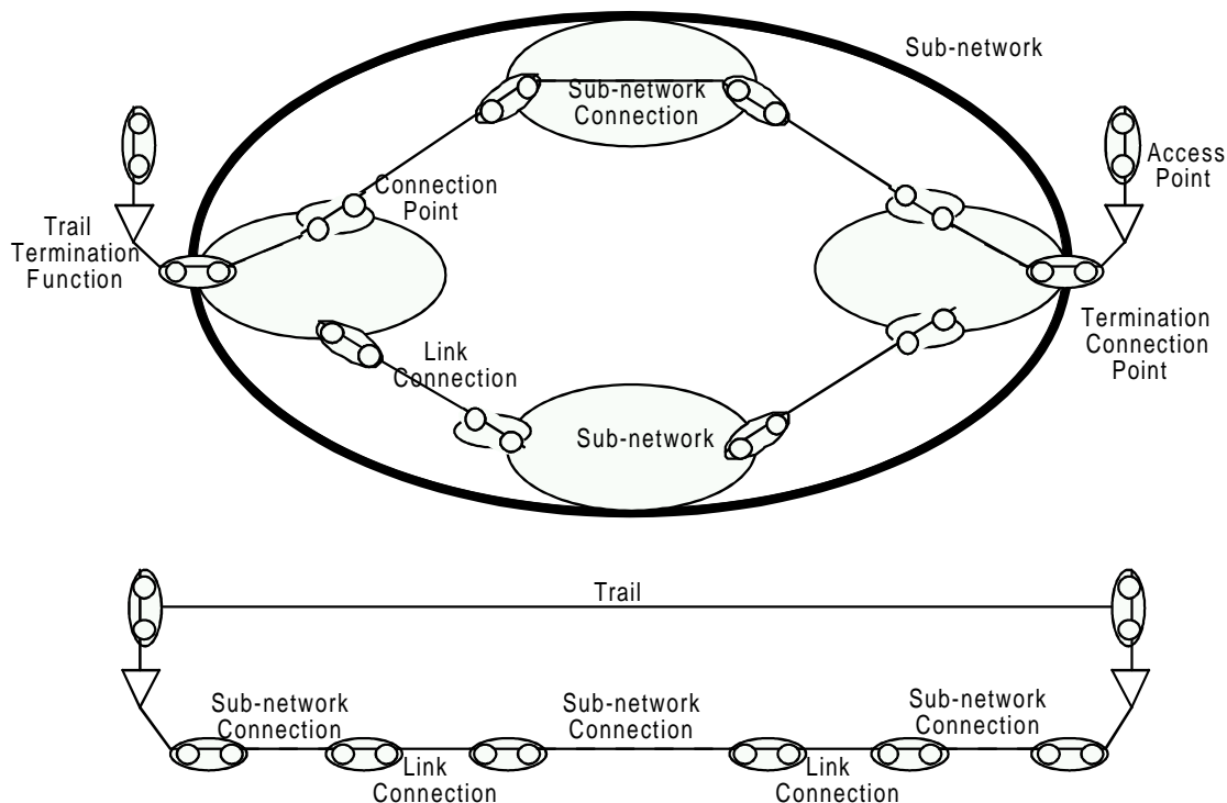
Figure 7: Single network element ring described in terms of ITU-T Recommendation G.803 [1] resources
