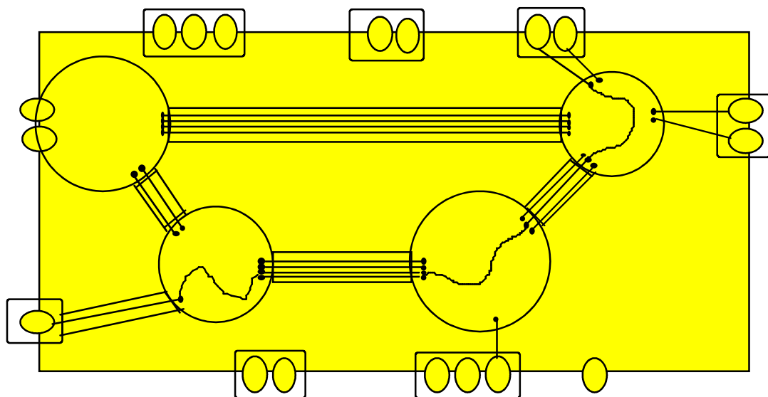
Figure 10: SNCs
