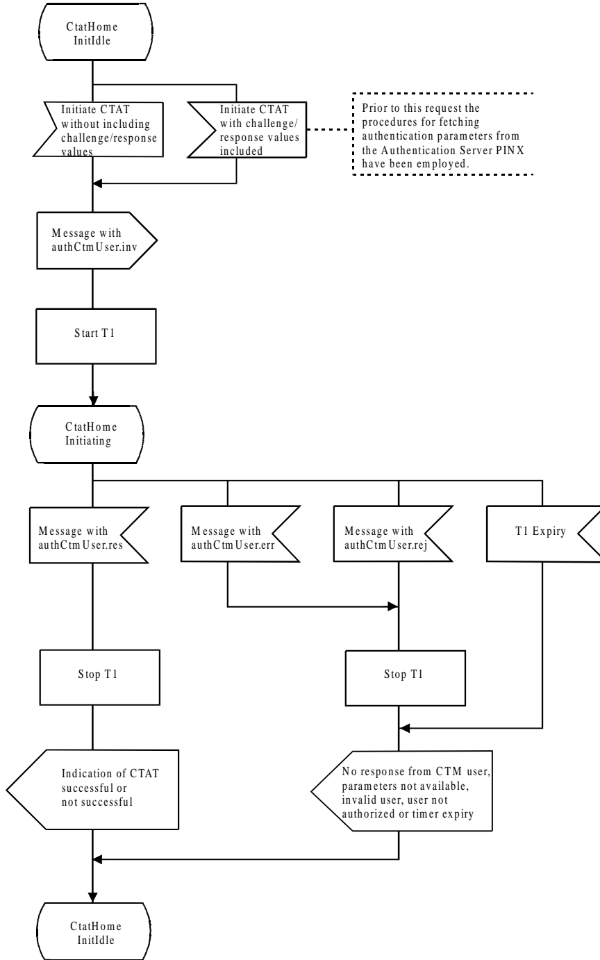
Figure C.1: SDL representation at the Home PINX for initiation of SS-CTAT
