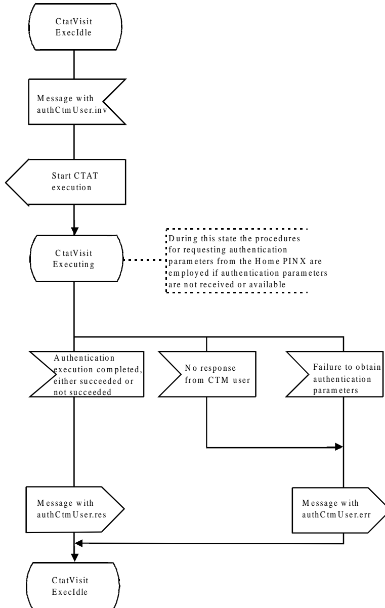
Figure C.4: SDL representation at the Visitor PINX for execution of SS-CTAT
