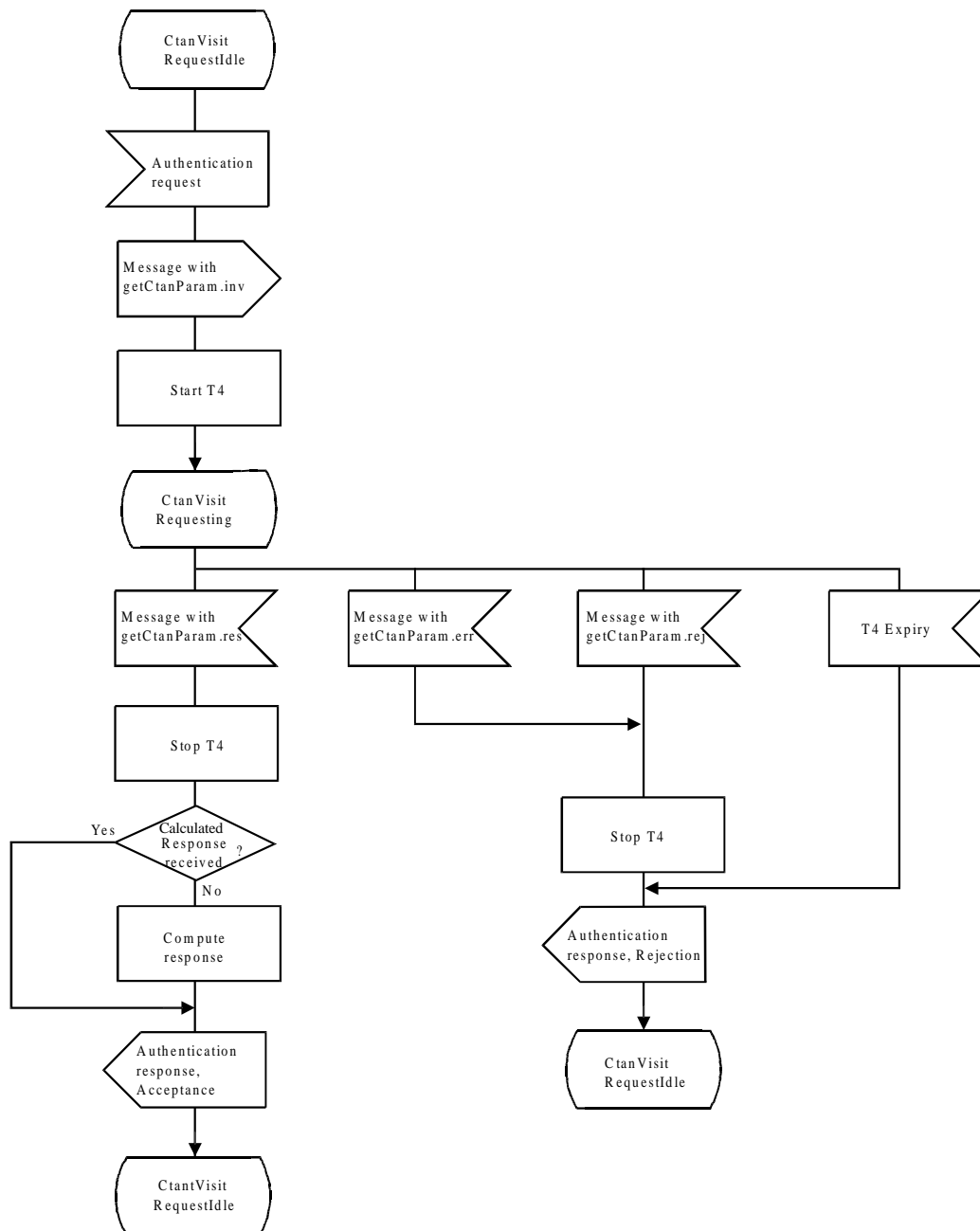
Figure C.7: SDL representation of SS-CTAN at the Visitor PINX
