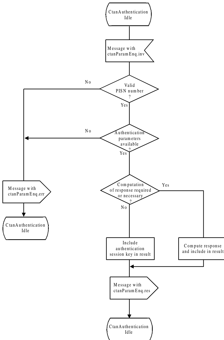
Figure C.9: SDL representation of SS-CTAN at the Authentication Server PINX
