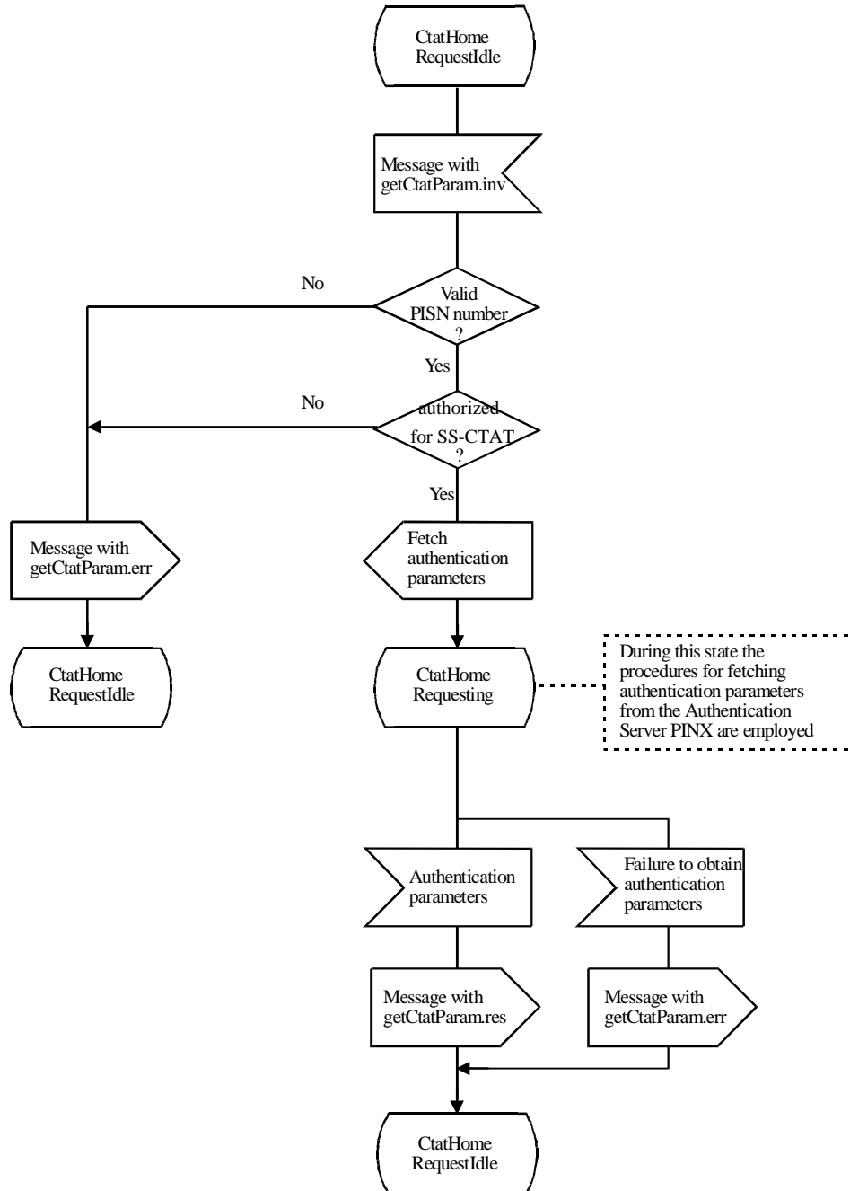
Figure C.2: SDL representation of SS-CTAT at the Home PINX for requesting authentication parameters
