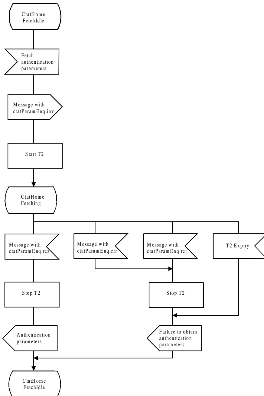
Figure C.3: SDL representation of SS-CTAT at the Home PINX when fetching authentication parameters
