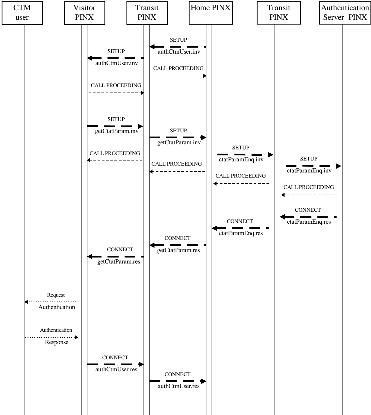
Figure B.2: Example message flow for authentication of a CTM user
