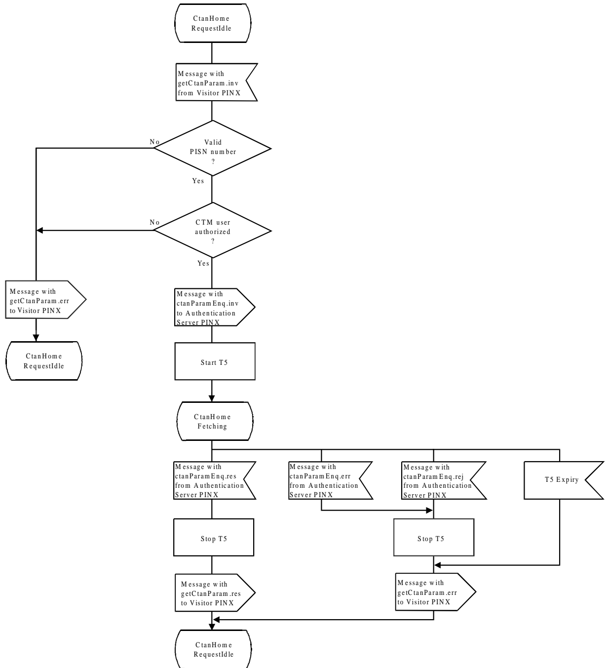
Figure C.8: SDL representation of SS-CTAN at the Home PINX
