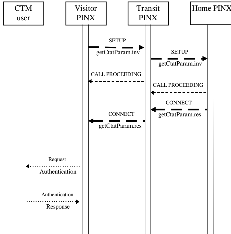
Figure B.1: Example message flow for authentication of a CTM user
