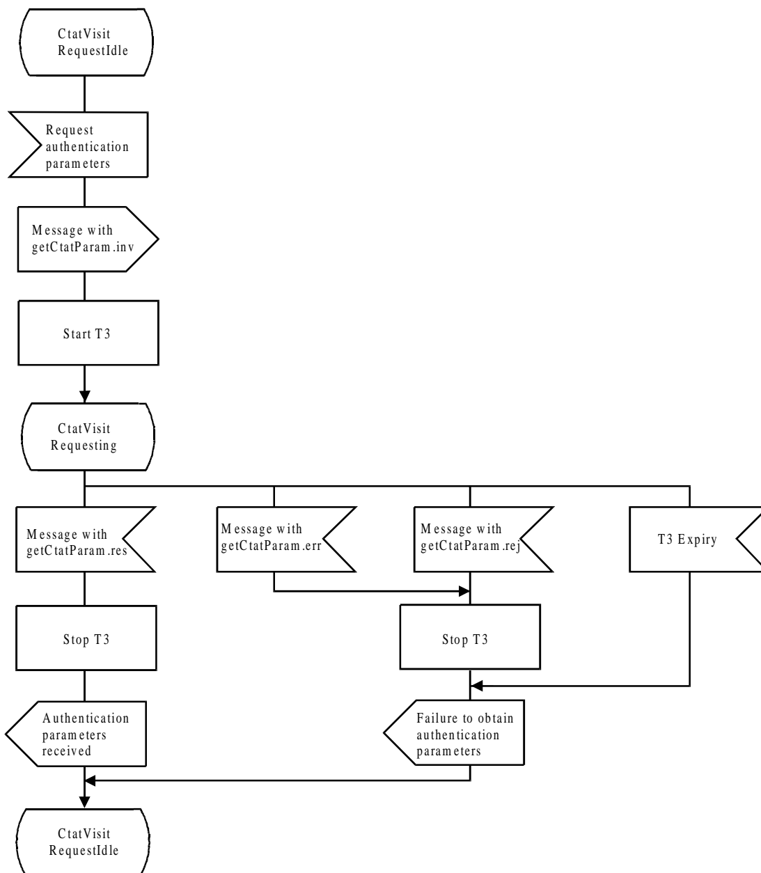
Figure C.5: SDL representation of SS-CTAT at the Visitor PINX for requesting authentication parameters
