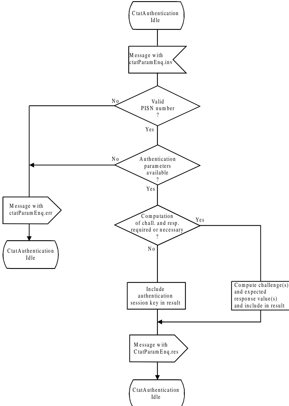
Figure C.6: SDL representation of SS-CTAT at the Authentication Server PINX
