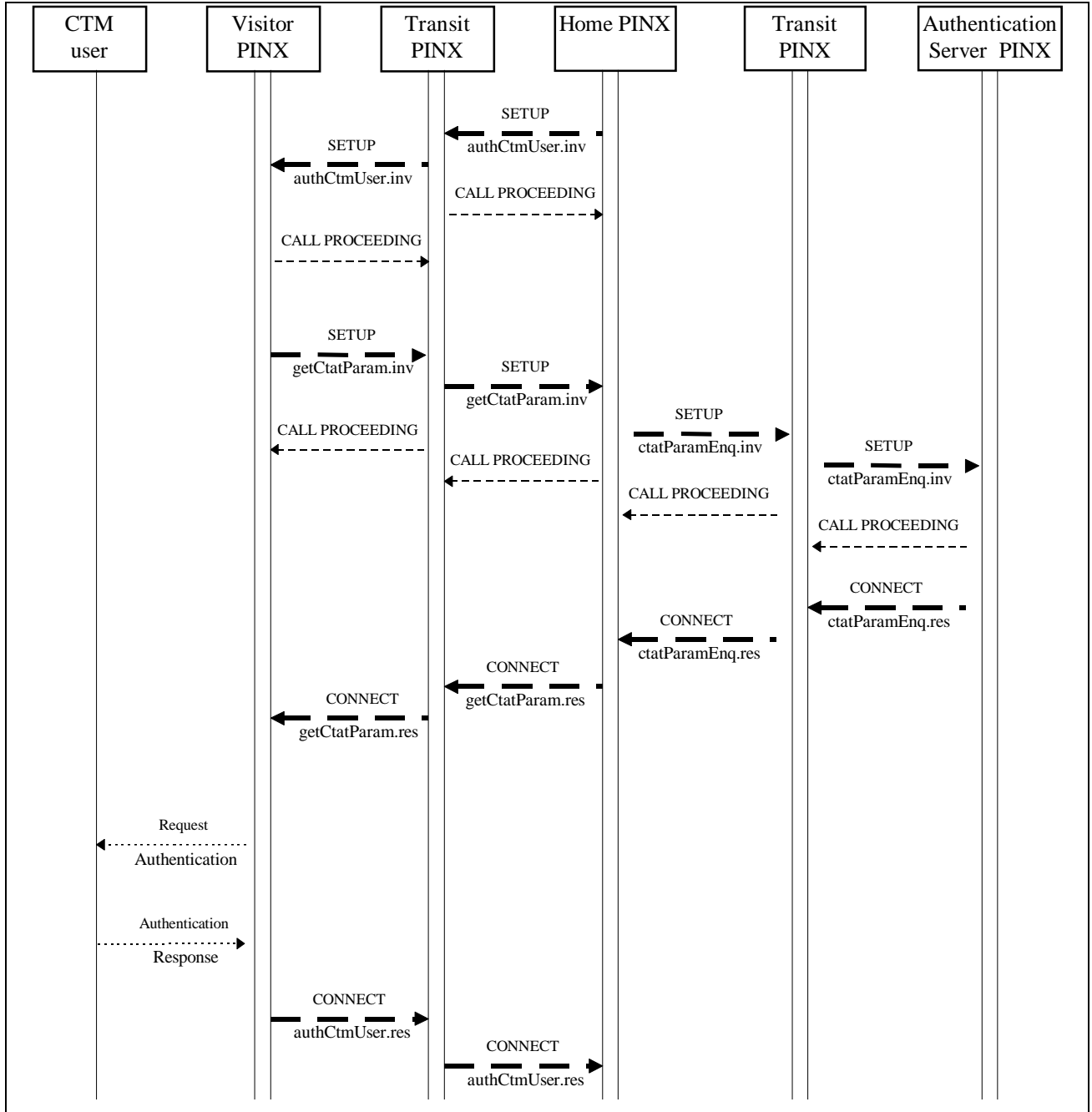
Figure B.2 - Example message flow for authentication of a CTM user
