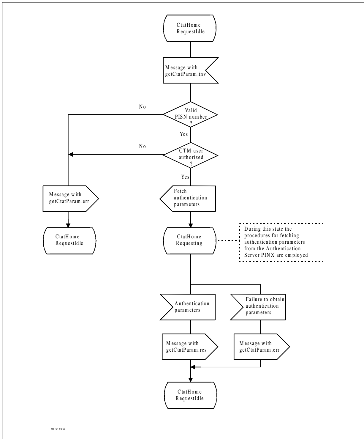
Figure C.2 - SDL representation of SS-CTAT at the Home PINX for requesting authentication parameters
