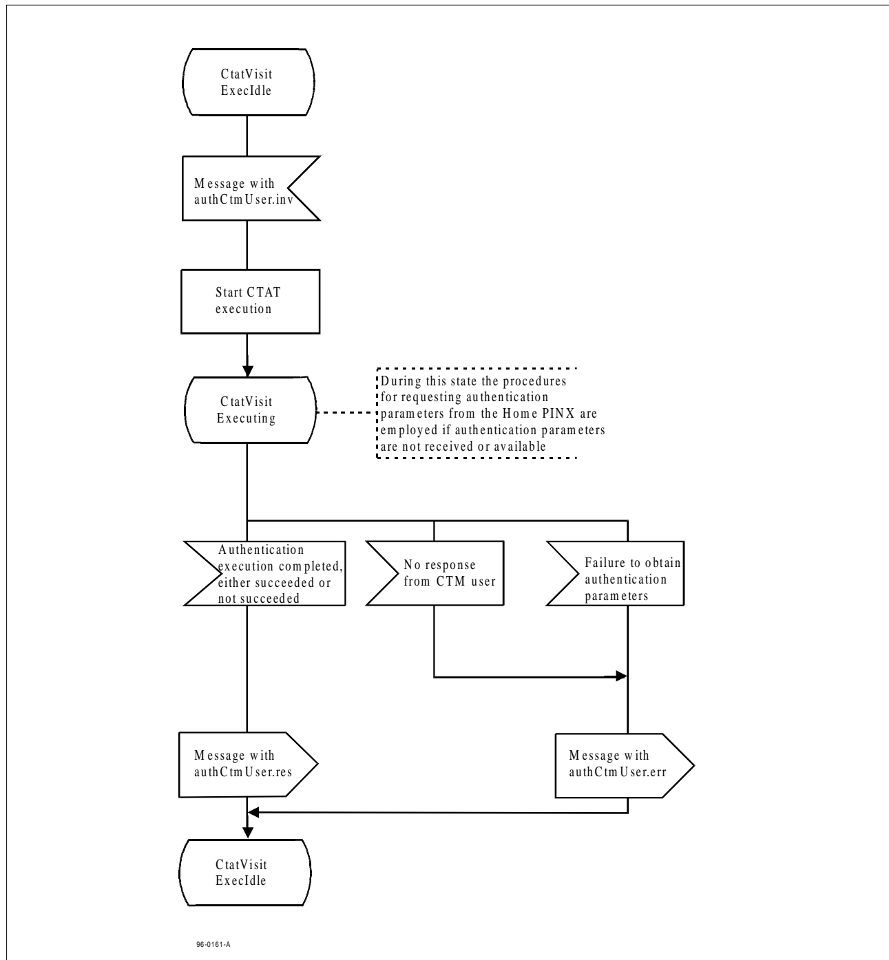
Figure C.4 - SDL representation at the Visitor PINX for execution of SS-CTAT
