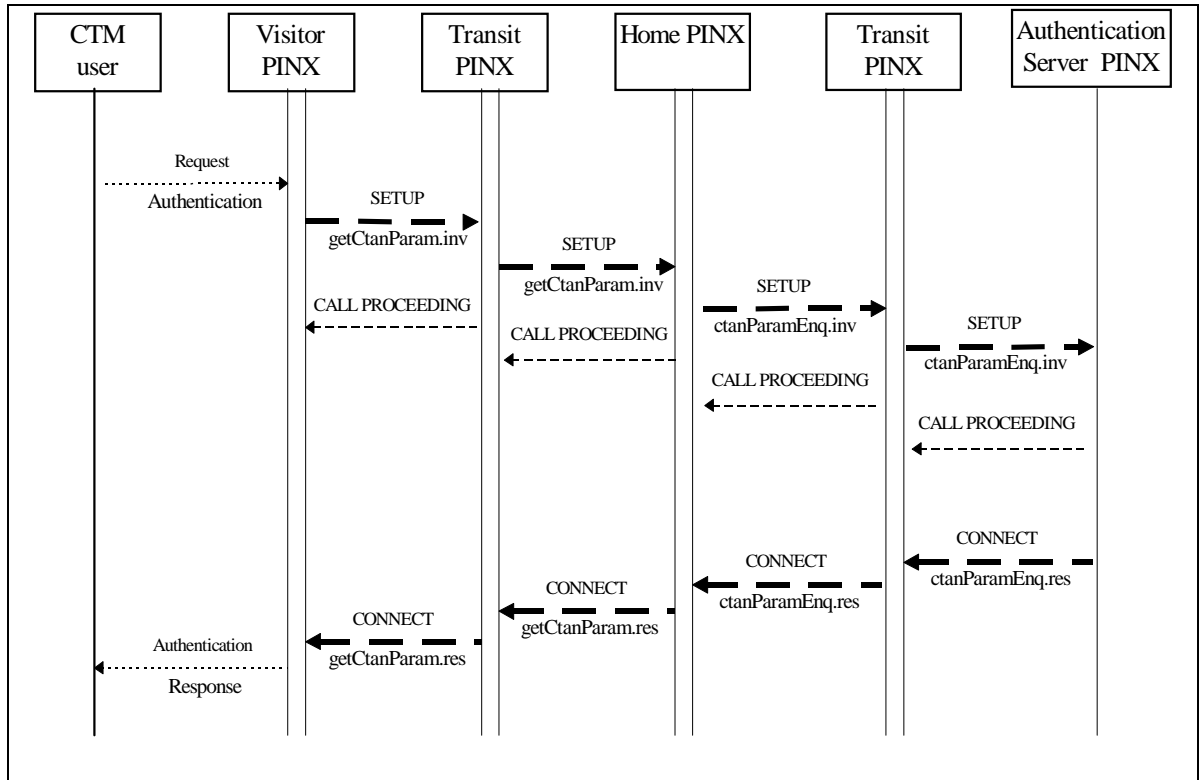
Figure B.4 - Example message flow for authentication of a PISN
