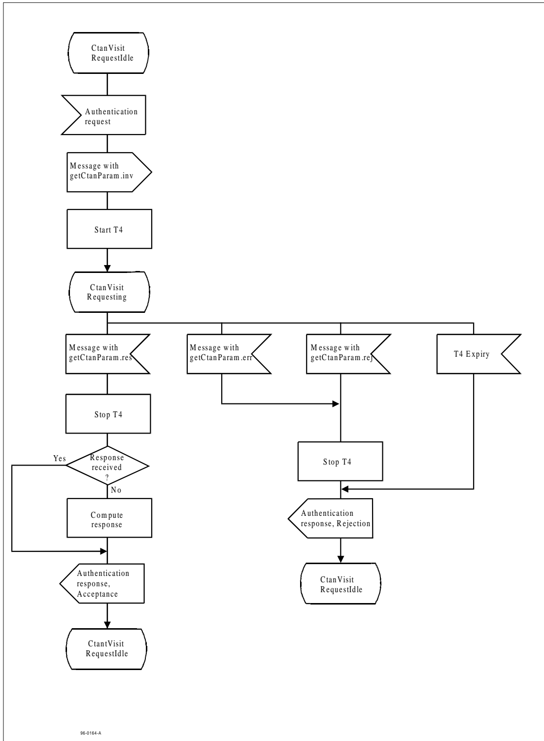
Figure C.7 - SDL representation of SS-CTAN at the Visitor PINX
