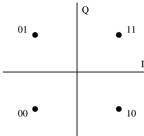
Figure 13: Mapping for the QPSK constellation (upstream)
