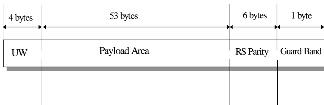
Figure 21: Slot format
