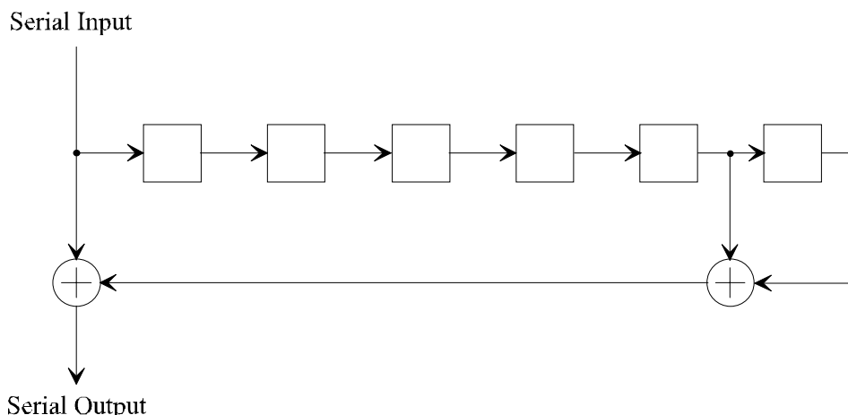
Figure 11: De-randomizer
