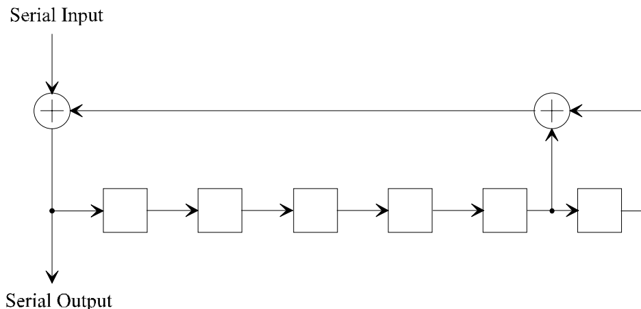
Figure 10: Randomizer
