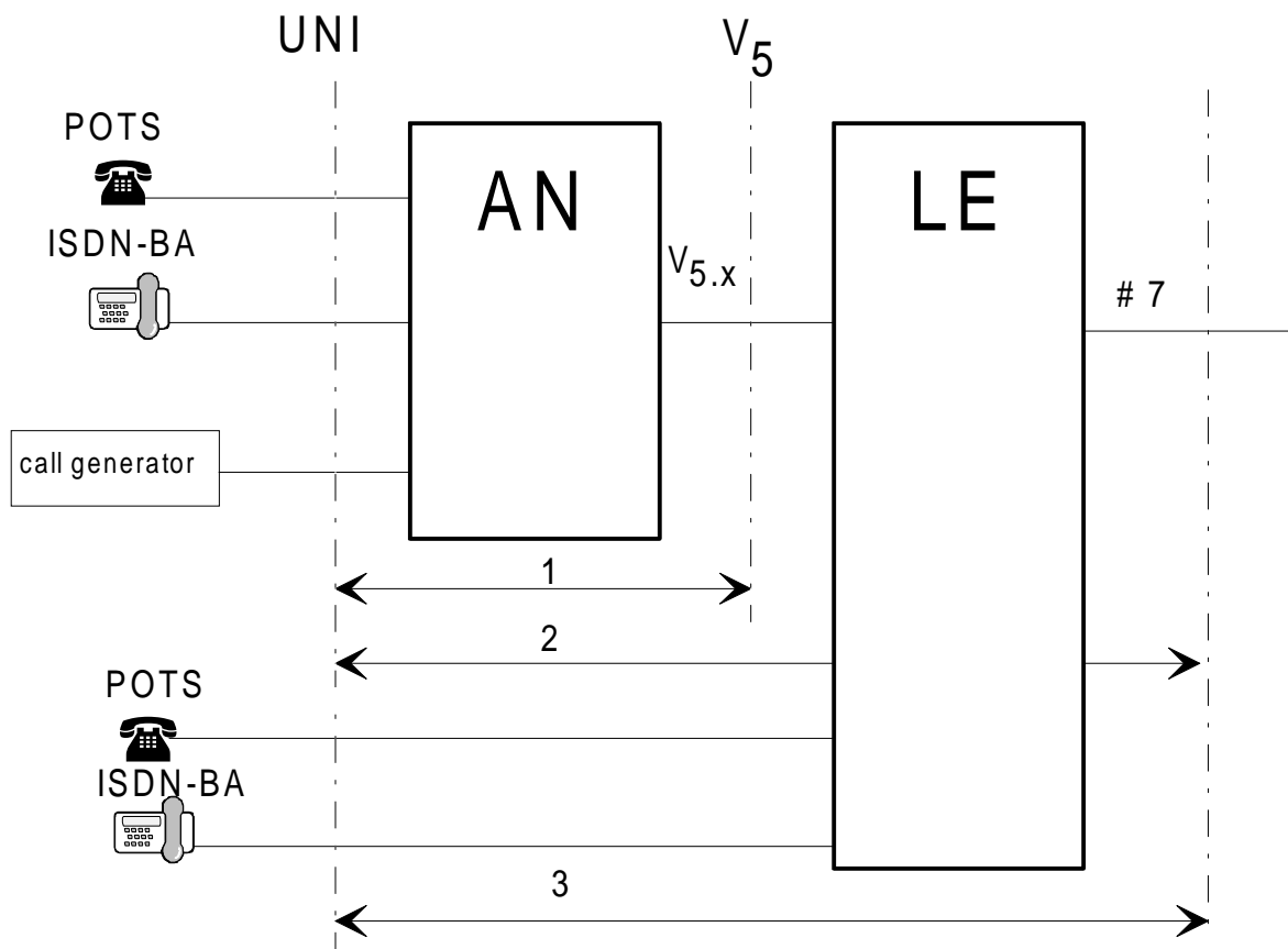
Figure C.5: measuring parts
