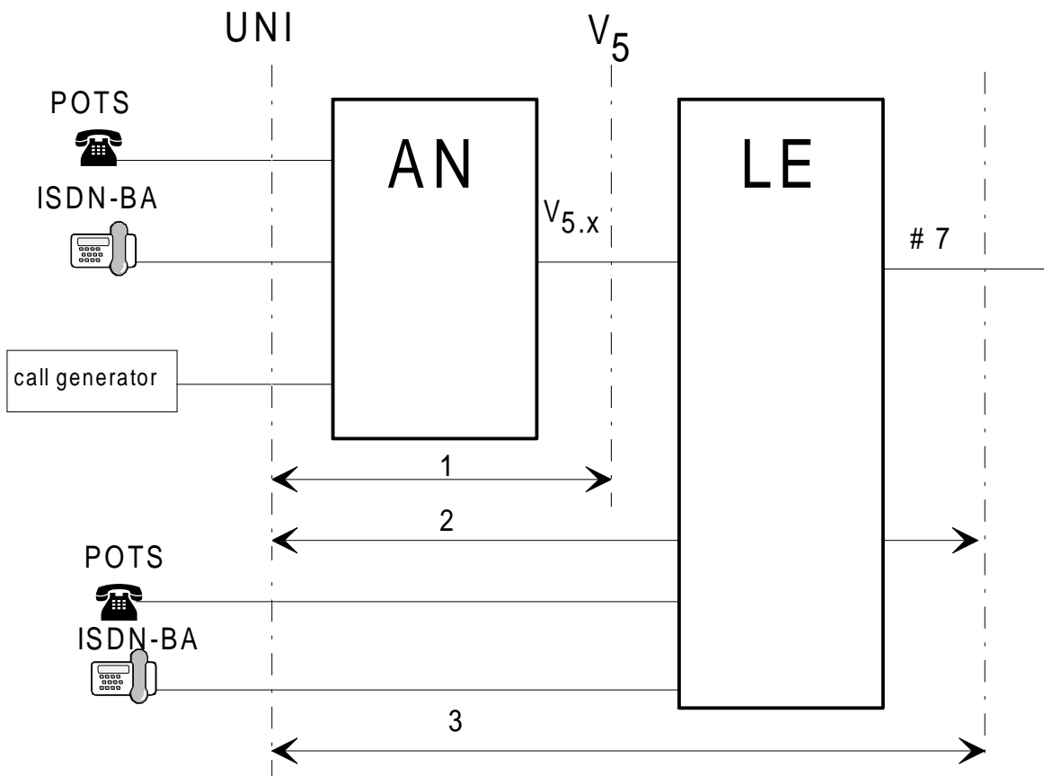
Figure C.5: measuring parts
