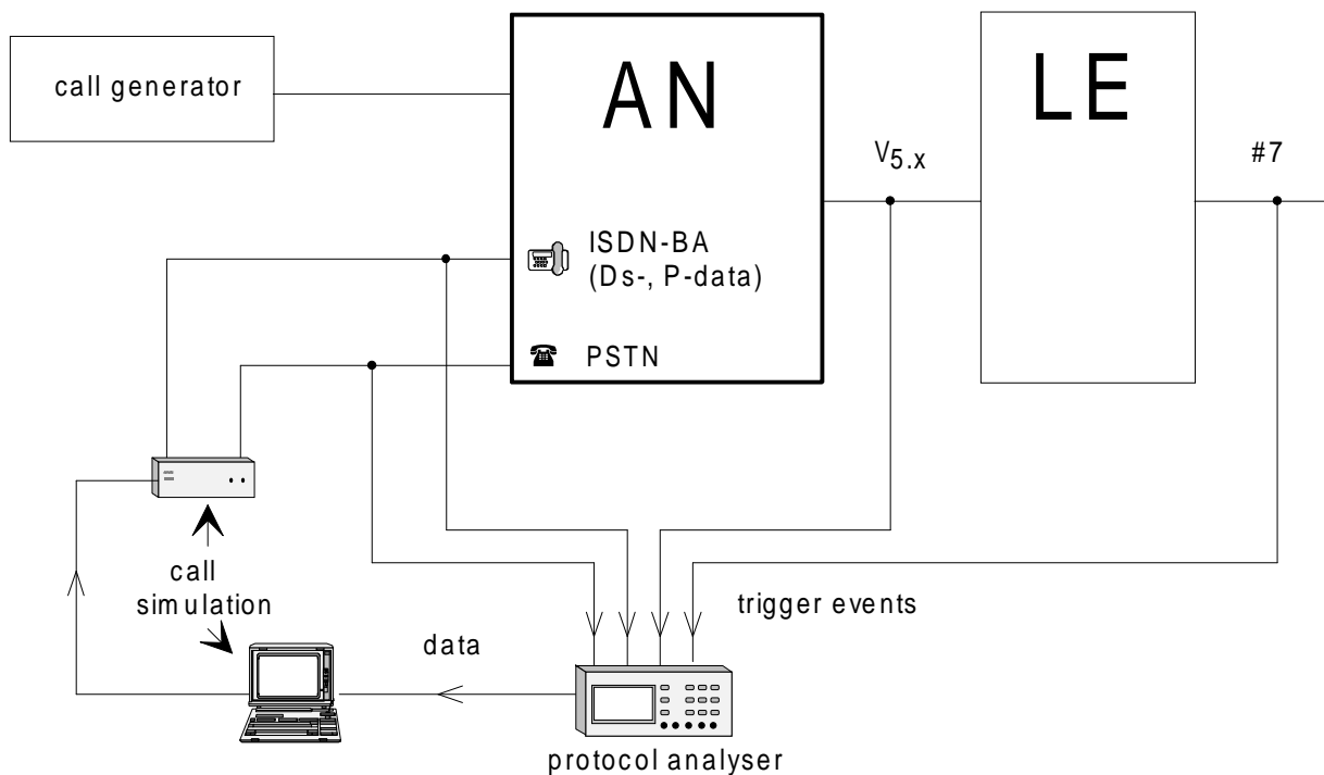
Figure C.6: Measuring set-up
