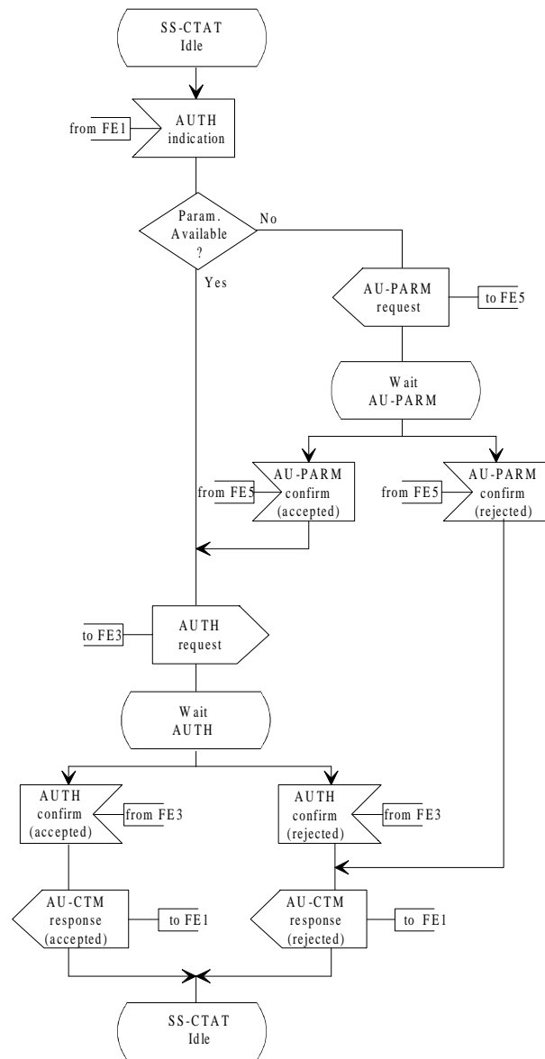
Figure 8: SDL for Functional Entity FE2
