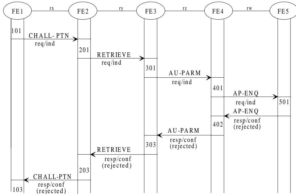
Figure 16: Unsuccessful case, rejection from FE5
