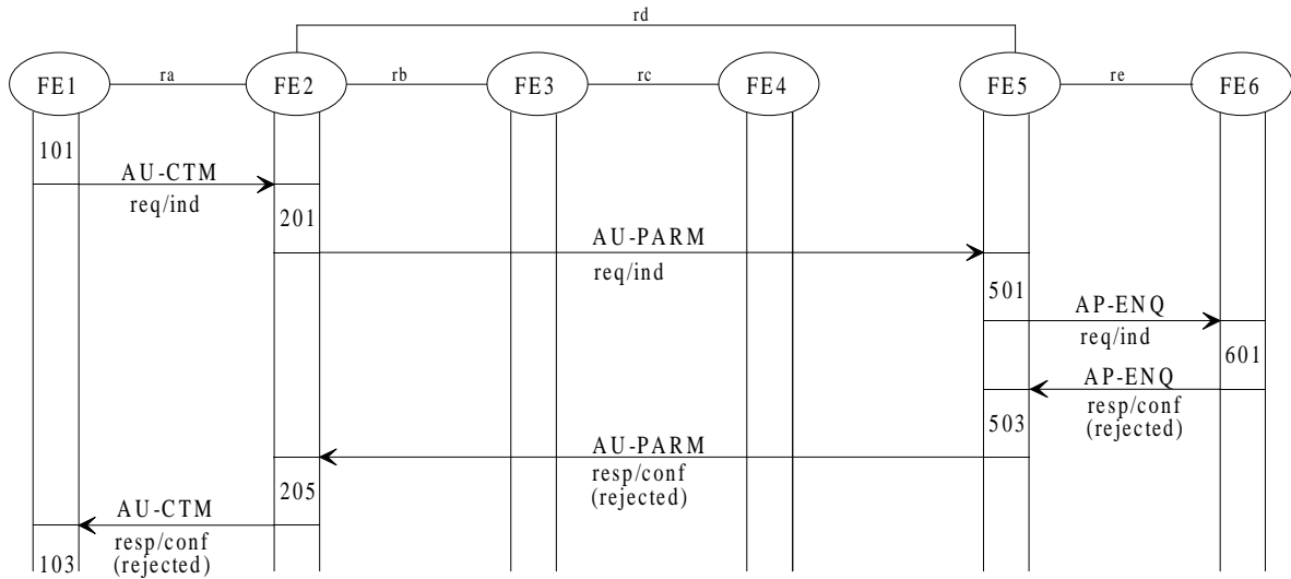
Figure 6: Unsuccessful case, rejection from FE6
