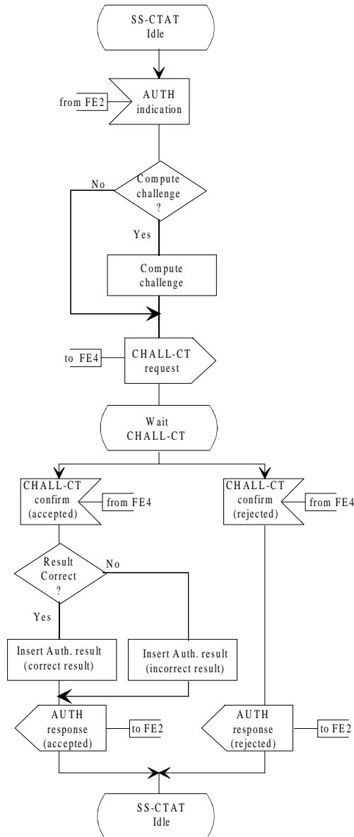
Figure 9: SDL for Functional Entity FE3
