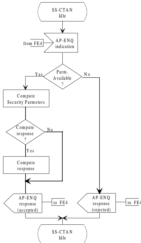
Figure 21: SDL for Functional Entity FE5
