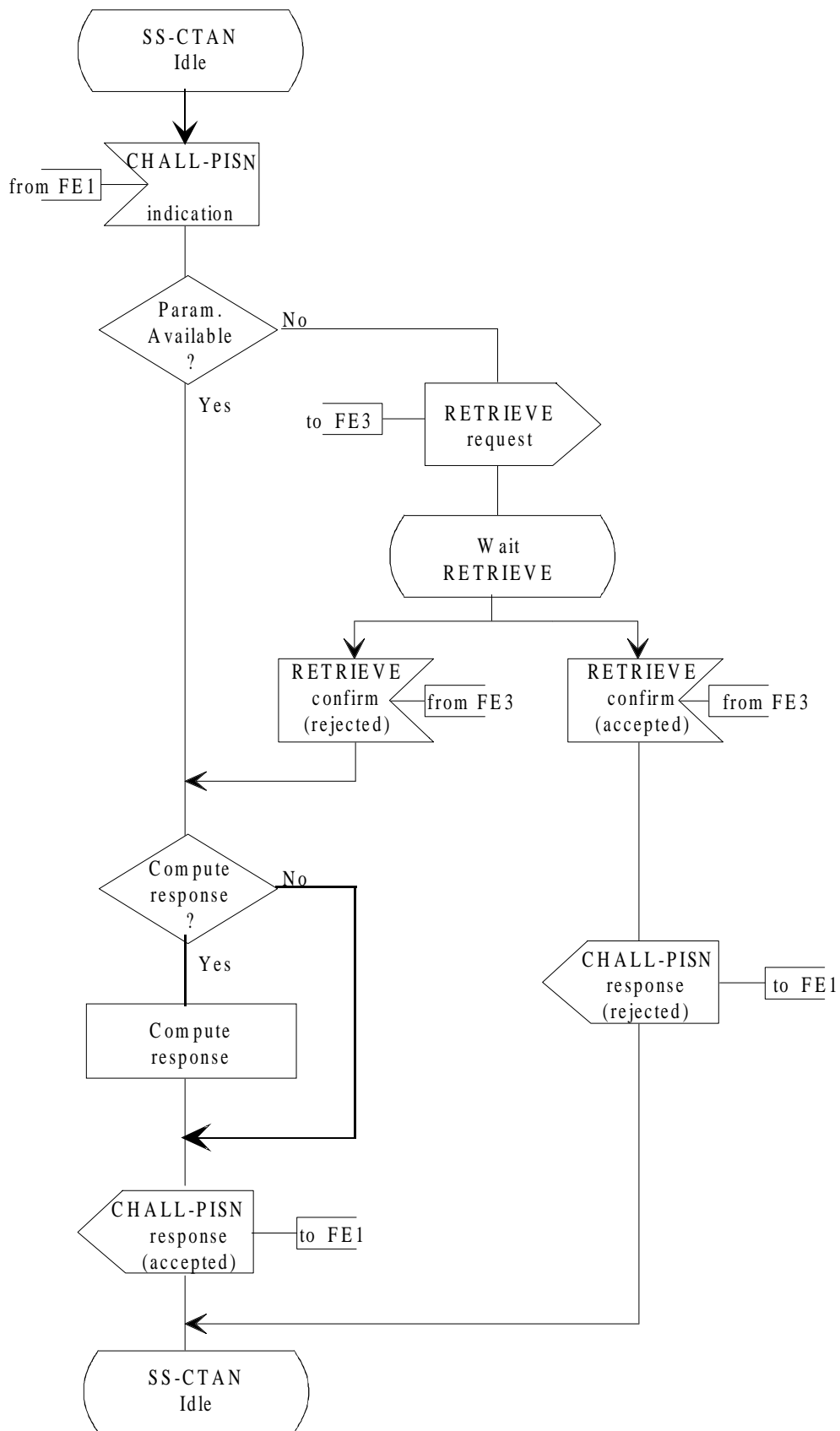
Figure 18: SDL for Functional Entity FE2
