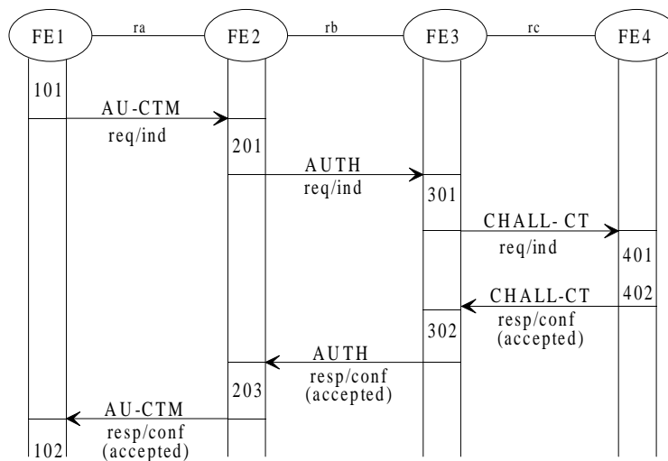
Figure 2: Successful case with parameters available locally in FE2
