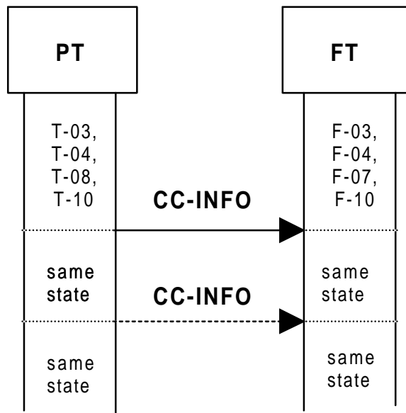
Figure 2: Sending on-hook information
