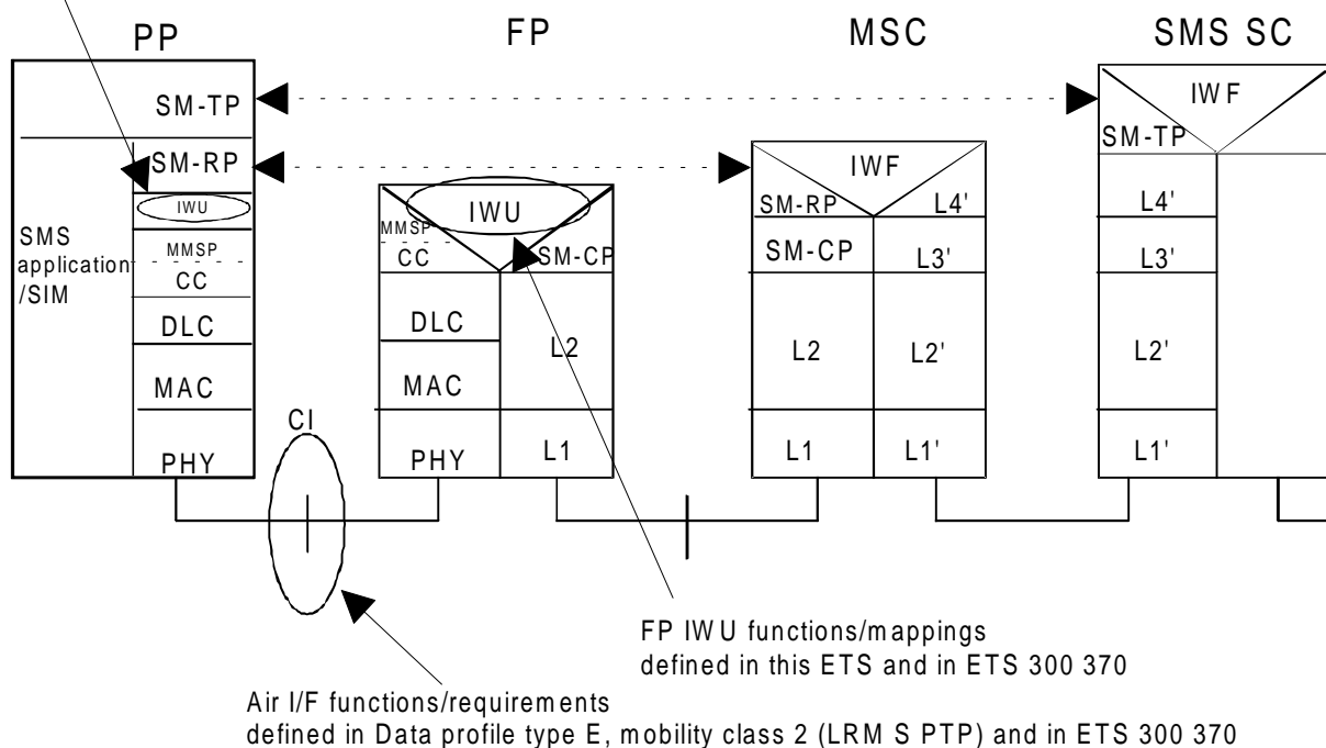
Figure 3: Interworking model of SMS, point-to-point, mobile originated and terminated (SM MO, SM MT) for FP GSM PLMN attachment
