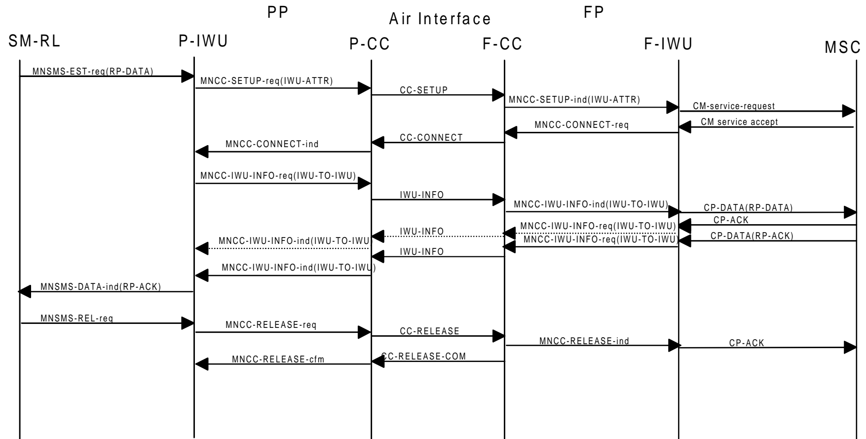
Figure D.1: Mobile originated SMS
