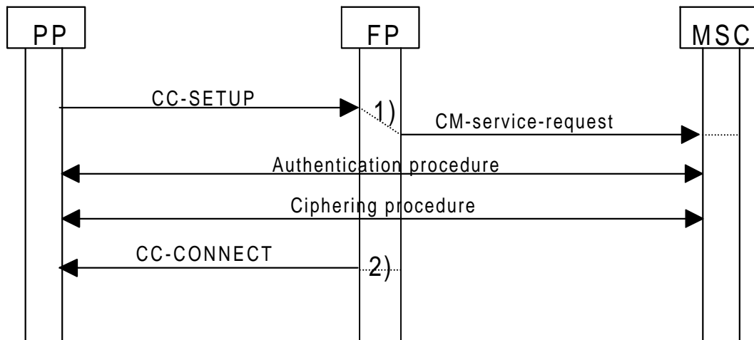
Figure 6: SM MO CM service procedure, with authentication and ciphering procedure
