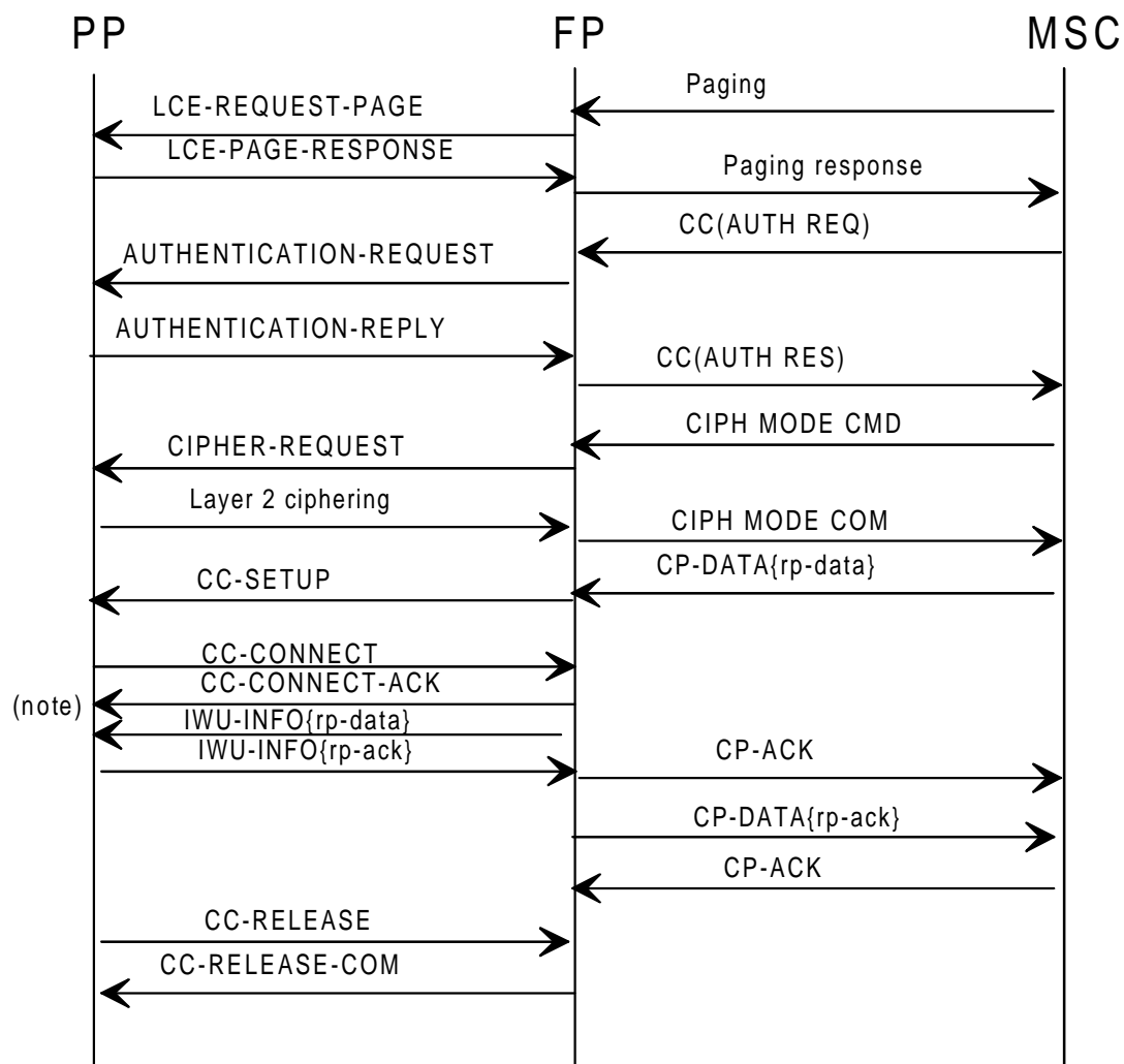
Figure C.2: Mobile terminated SMS (DECT/GSM interworking) - CP layer interworking
