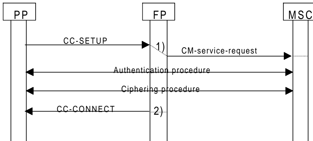
Figure 6: SM MO CM service procedure, with authentication and cipherring procedure
