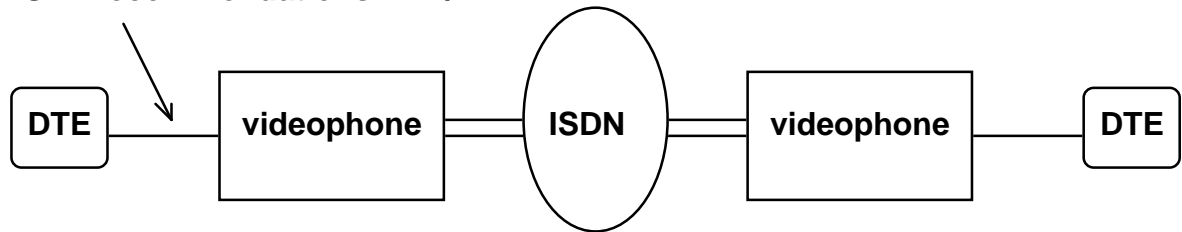
Figure 1: System configuration
