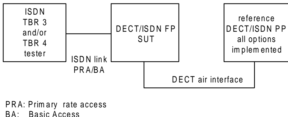
Figure 4: ISDN protocols testing at FT
