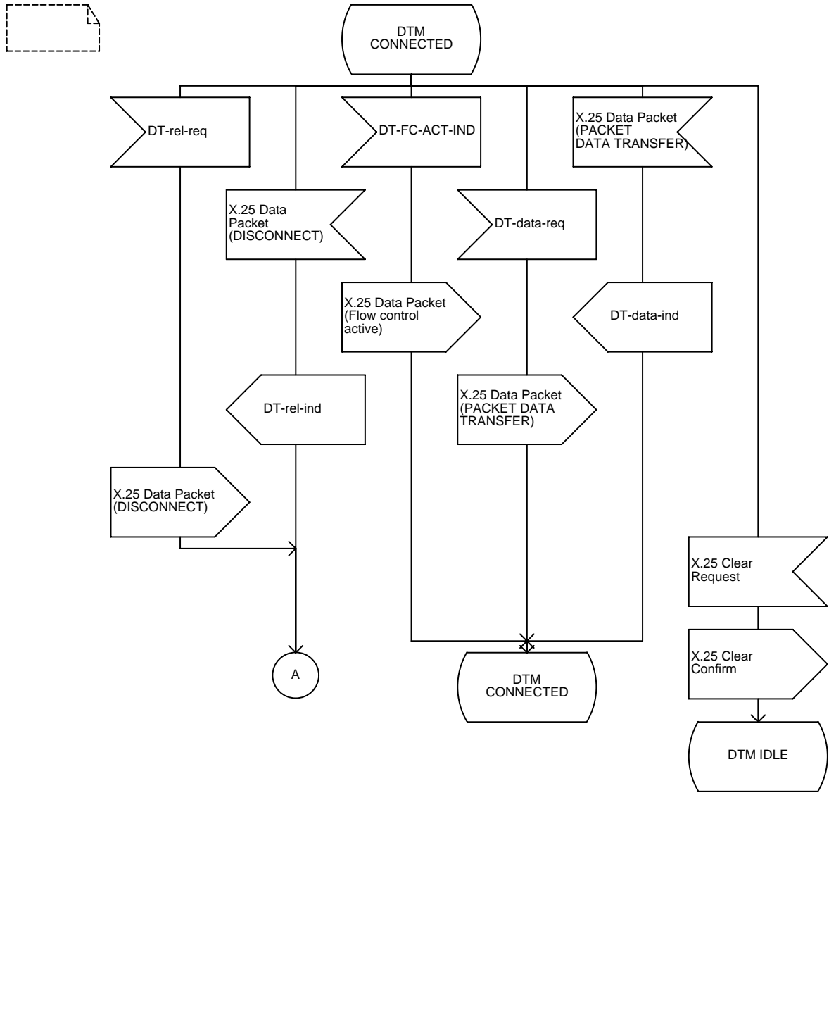
Figure C.4: (sheet 3 of 5) DTM GSS protocol CIF side
