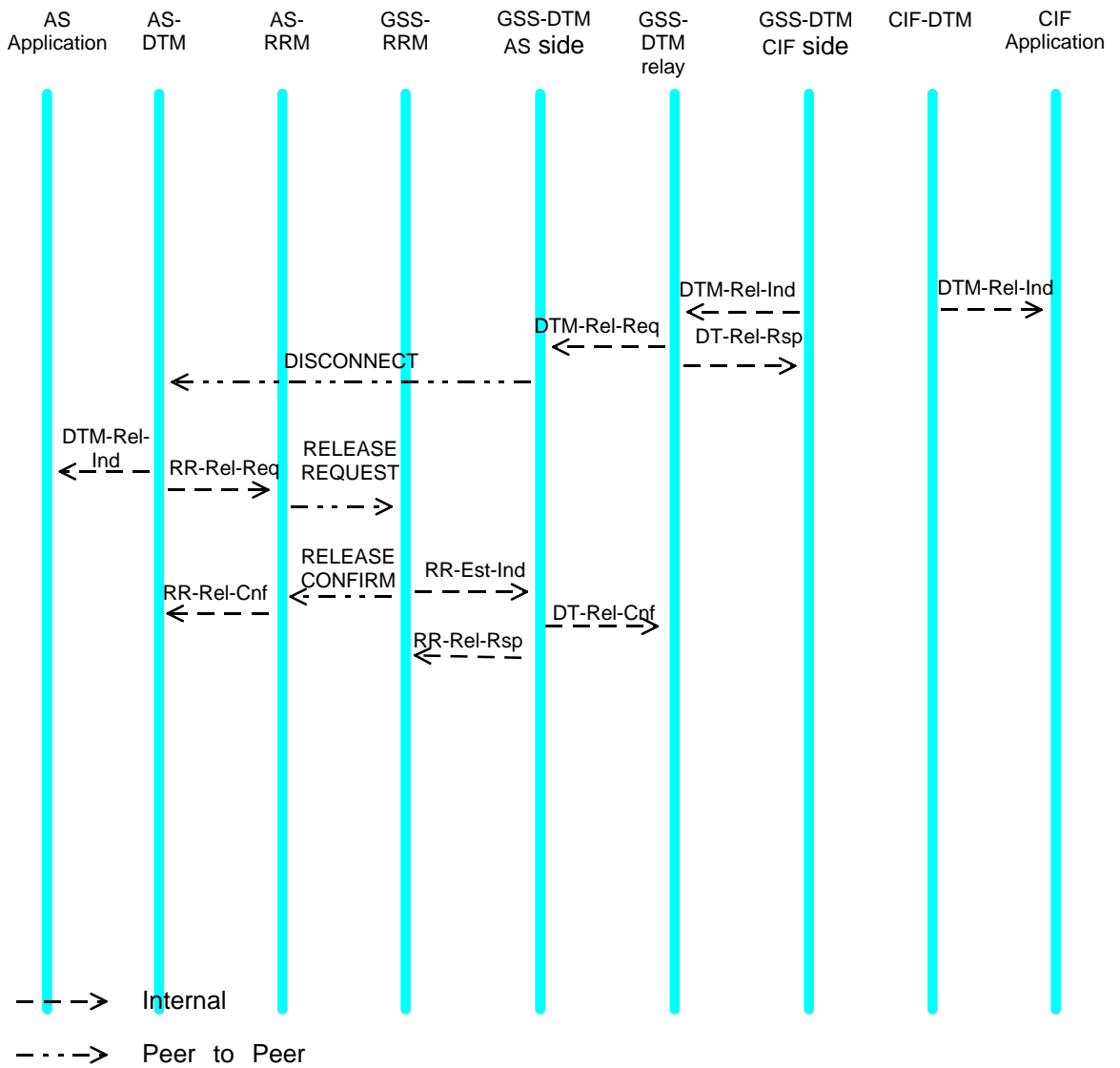
Figure B.14: Transaction release. GSS-CIF data link failure
