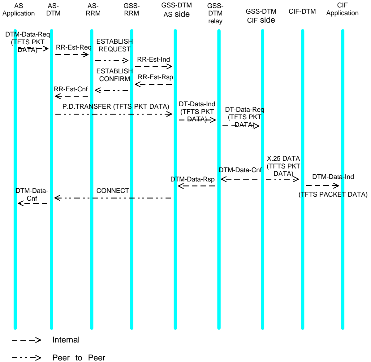
Figure B.2: Transaction establishment. AT originating, GSS-CIF connected
