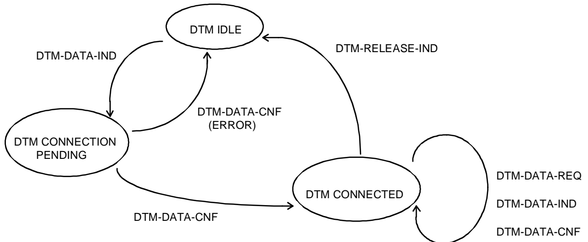
Figure 10: Overview service state diagram of the DTM entity on the GSS side
