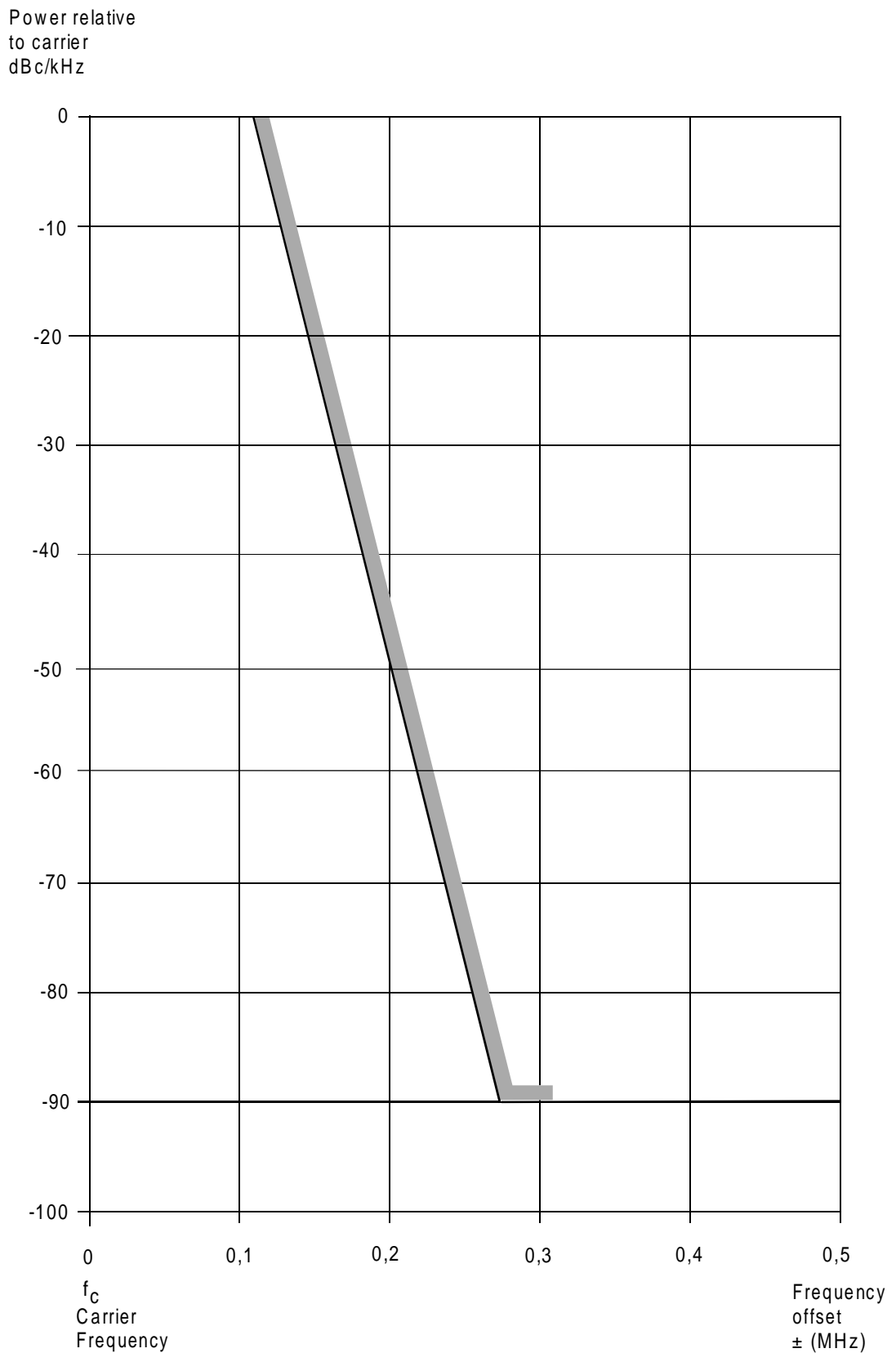
Figure 4: Limits on transmitter spectrum due to abnormal AF input levels (see subclause 4.9)
