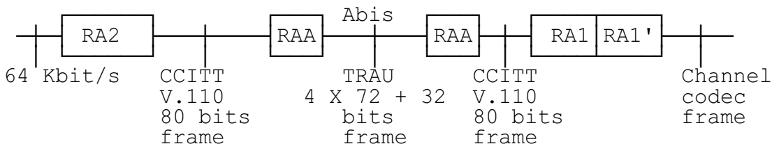
Figure GSM 08.60/4.3: Rate adaption when 16 kbit/s traffic channels are used.
